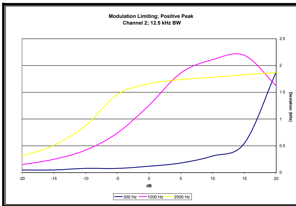
PLOT 8-1: MODULATION LIMITING RESPONSE (NARROWBAND POSITIVE PEAK), CH 2, 480 MHZ
