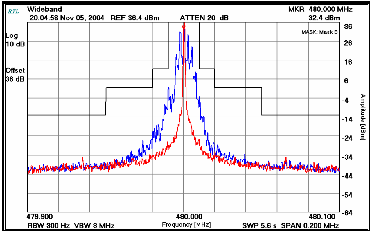
PLOT 9-2: MASK B (480 MHZ; CH 2; WIDEBAND)
