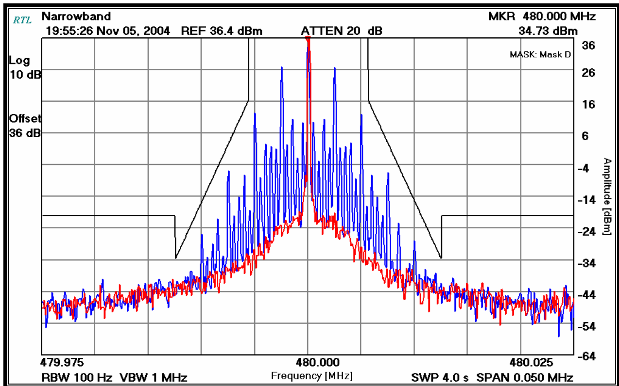
PLOT 9-1: MASK D (480 MHz; CH 2; NARROWBAND)
