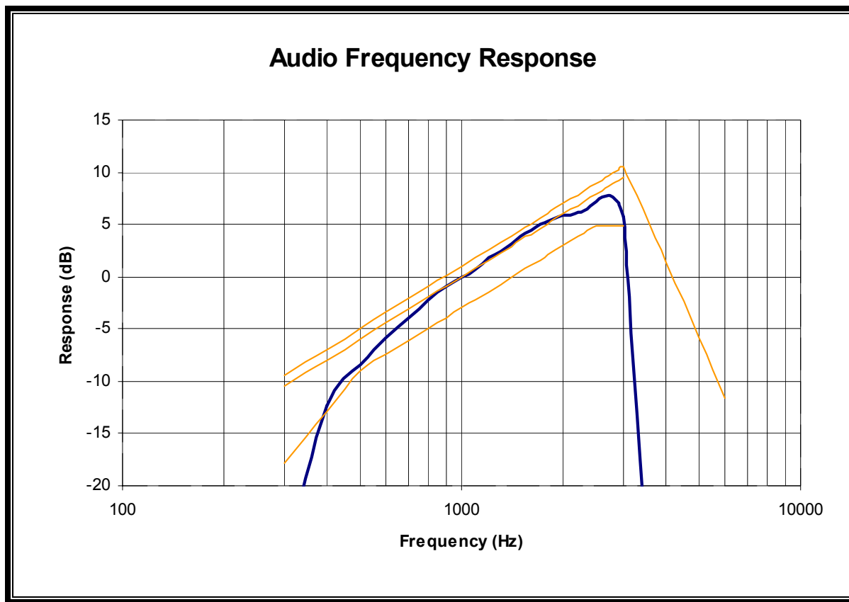
PLOT 6-1: AUDIO FREQUENCY RESPONSE
