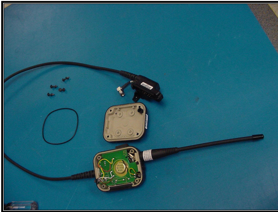
PHOTOGRAPH 5: SPEAKER/MICROPHONE WITH ANTENNA WITH CABLE
