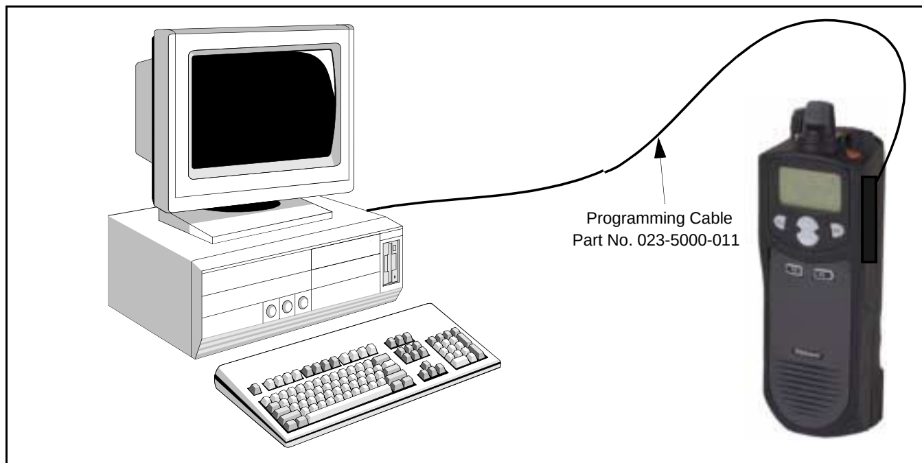
Figure 3-1 Programming Setup
