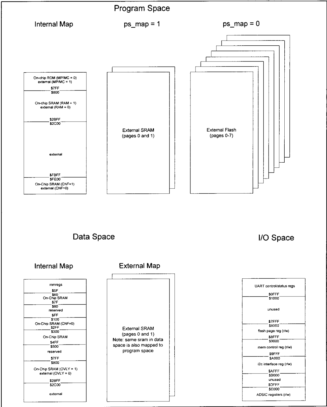
Figure 5-2 Memory Utilization
