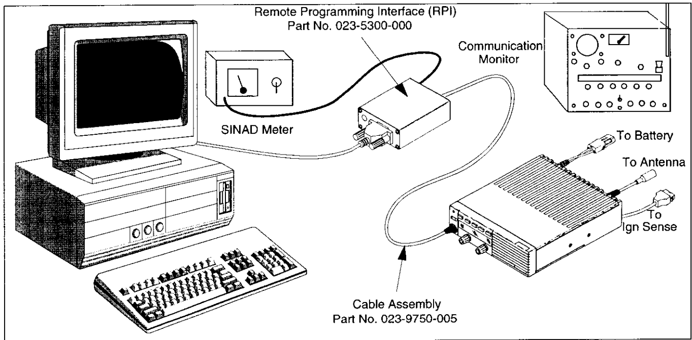
Figure 6-1 Alignment Setup
