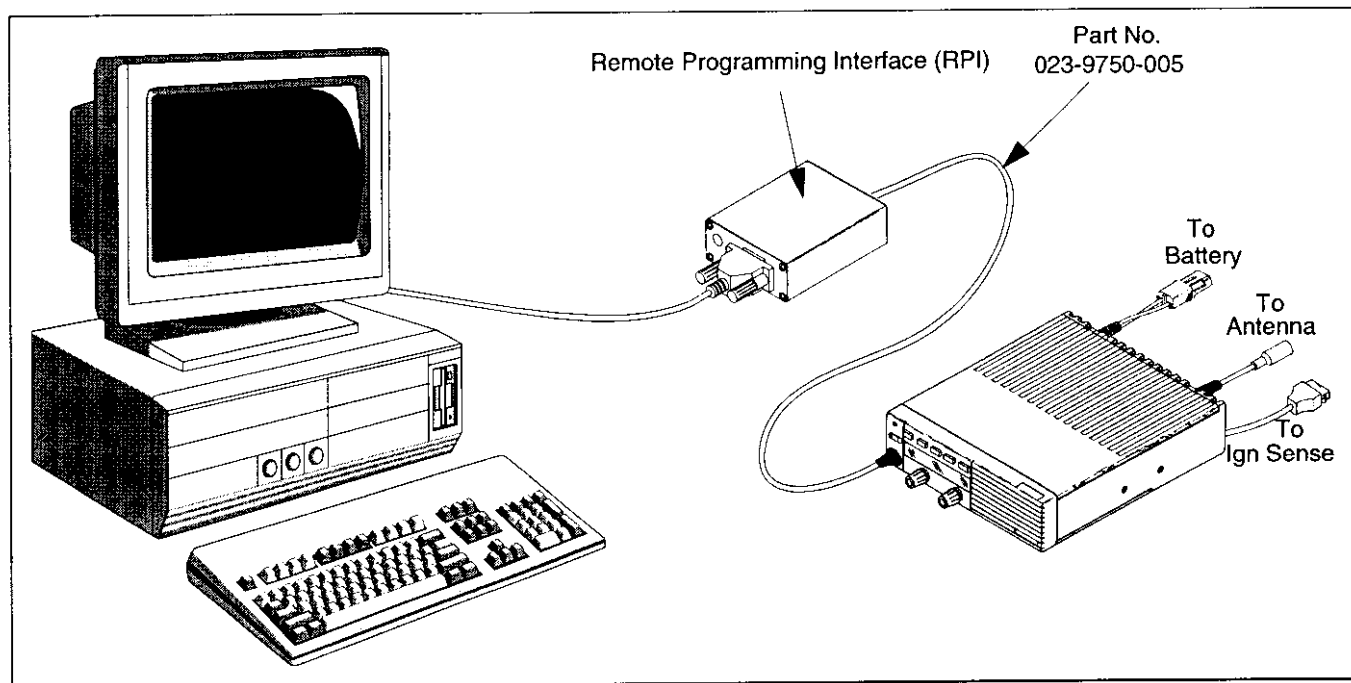
Figure 4-1 Programming Setup
