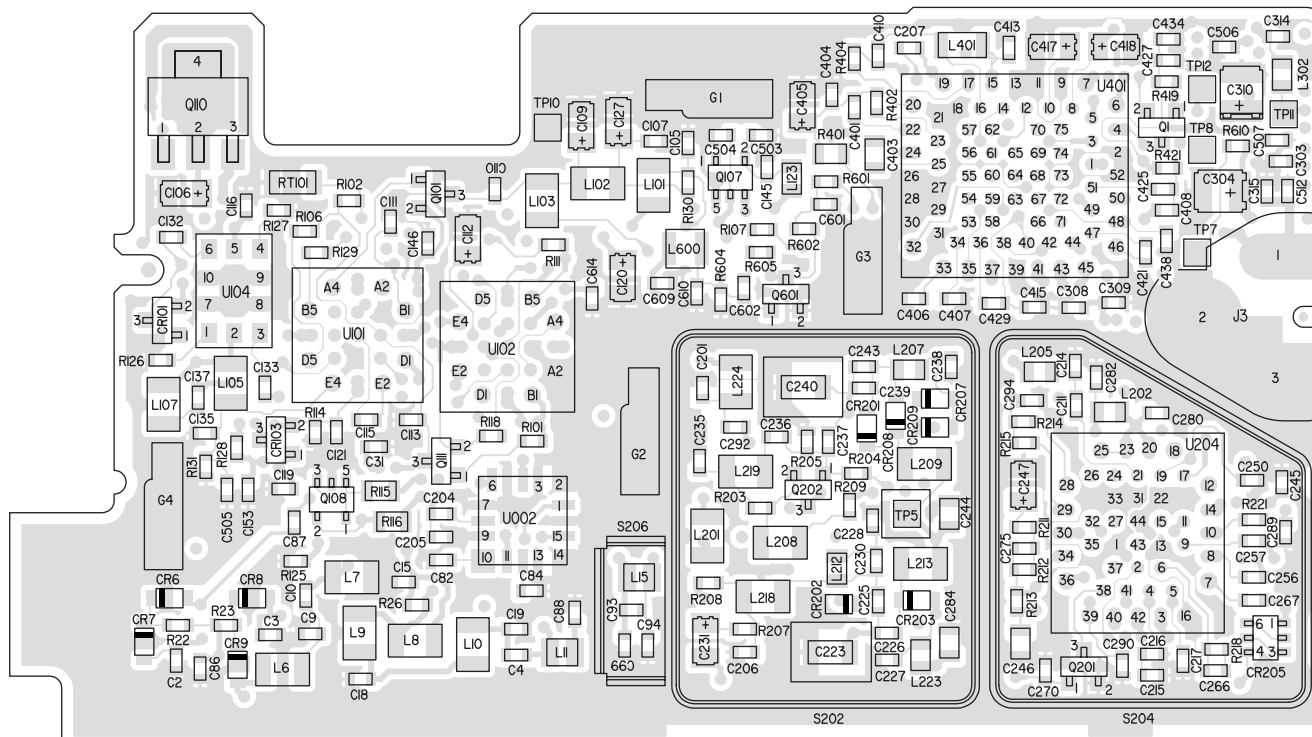
BOTTOM VIEW
