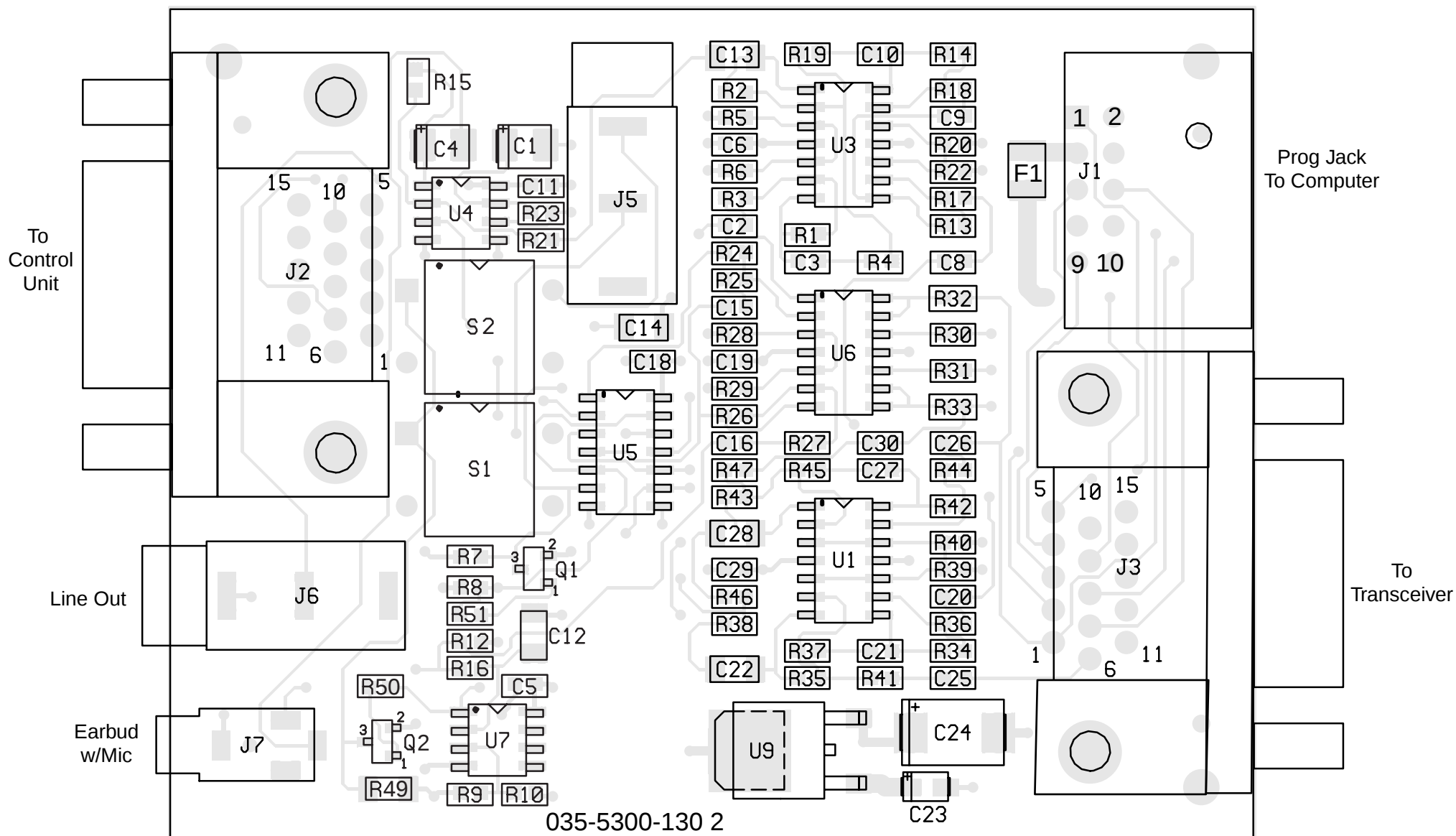
HANDHELD CONTROL UNIT JUNCTION BOX BOARD
