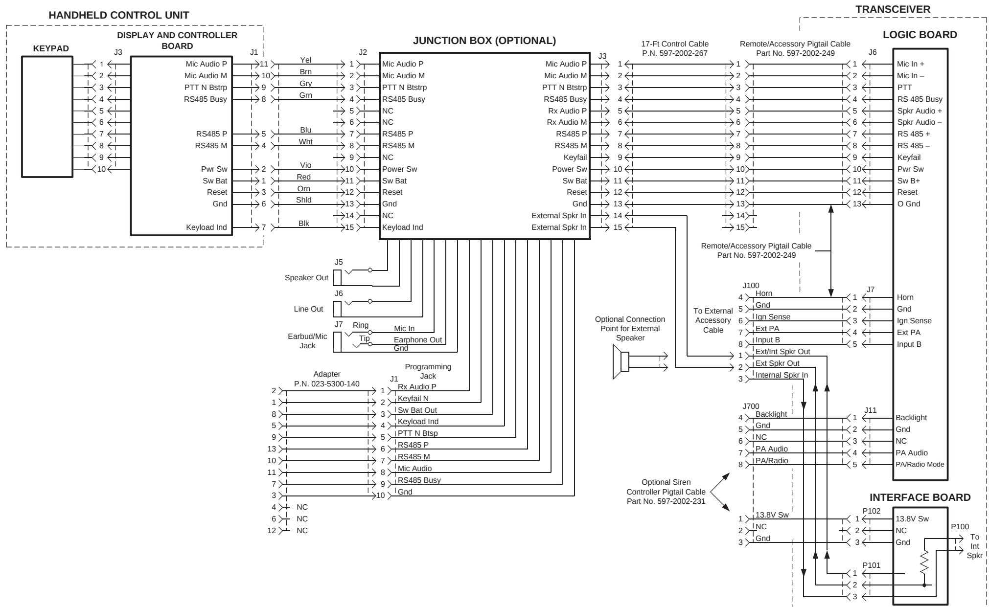
HANDHELD CONTROL UNIT INTERCONNECT SCHEMATIC
