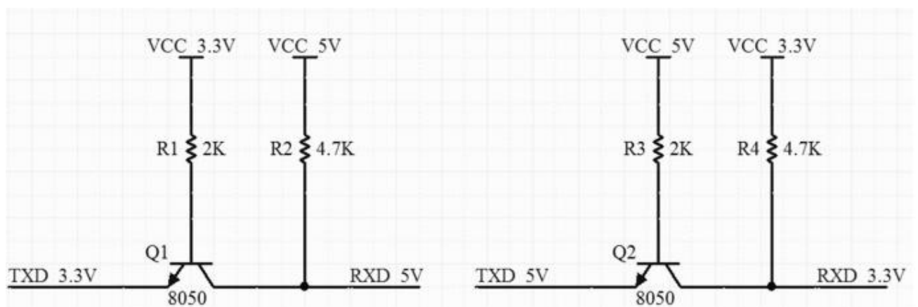
Figure 4.2 GPIO Level Conversion
