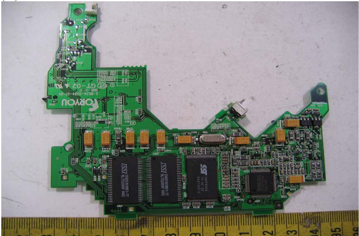
(14) Solder View of LCD Panel 's PCB
