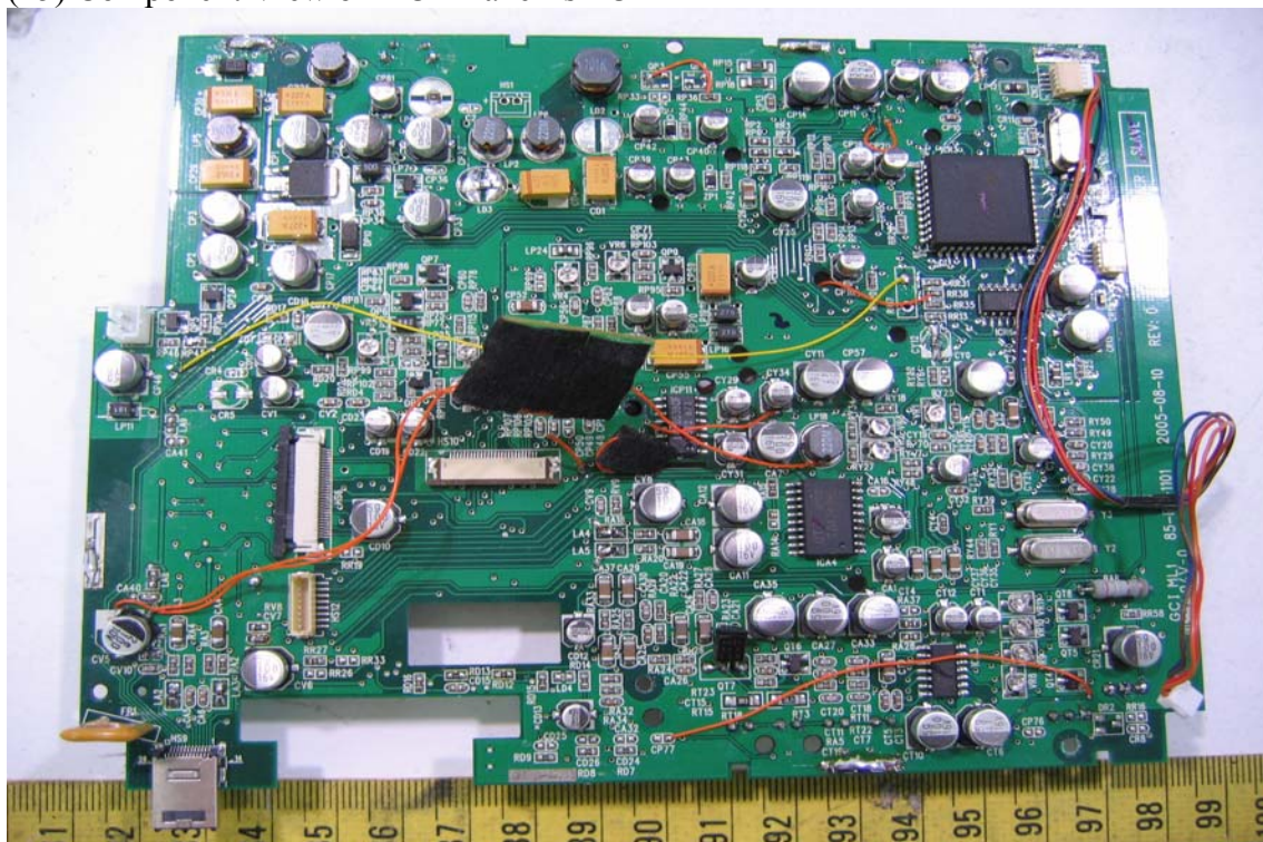
(15) Component View of LCD Panel 's PCB
