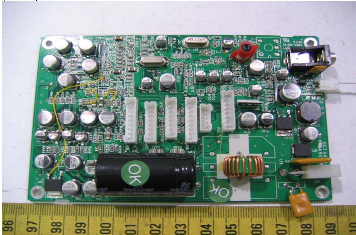
(6) Component View of the PCB
