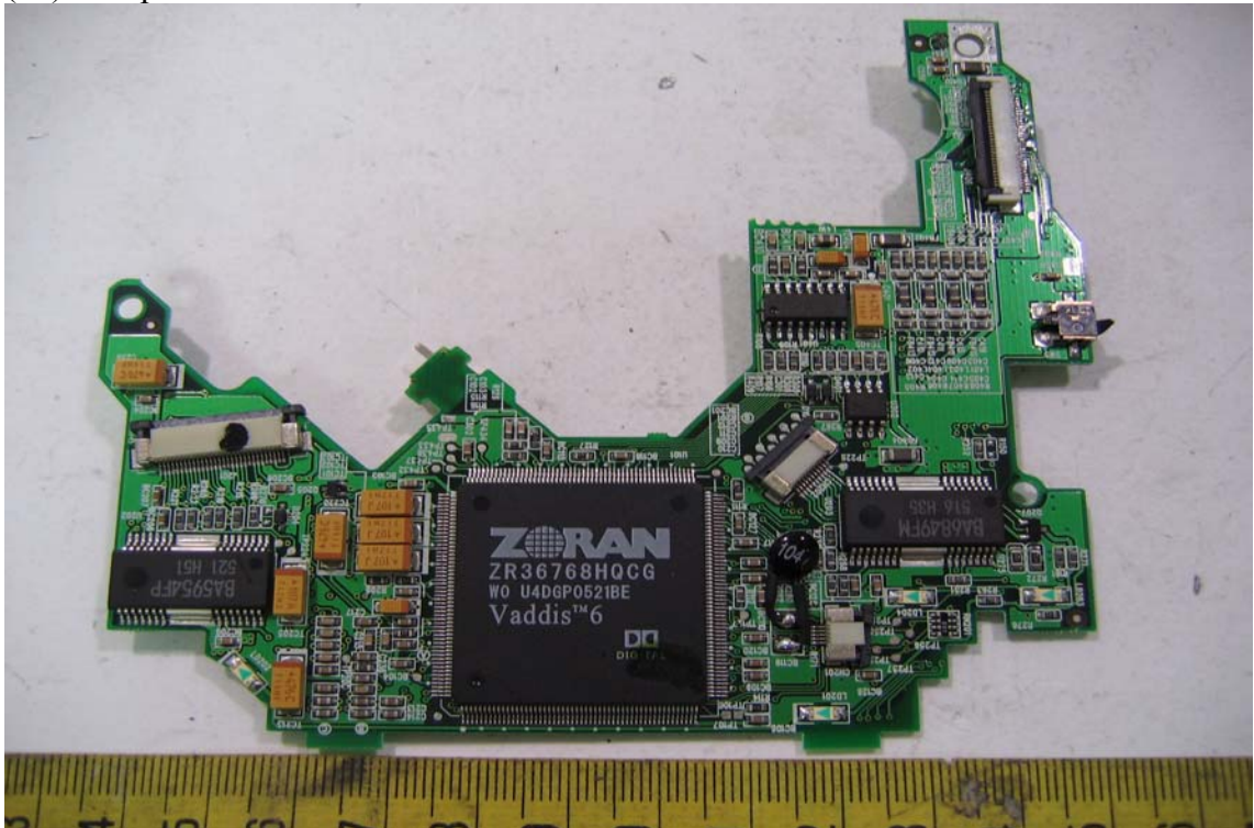
(13) Component View of LCD Panel 's PCB
