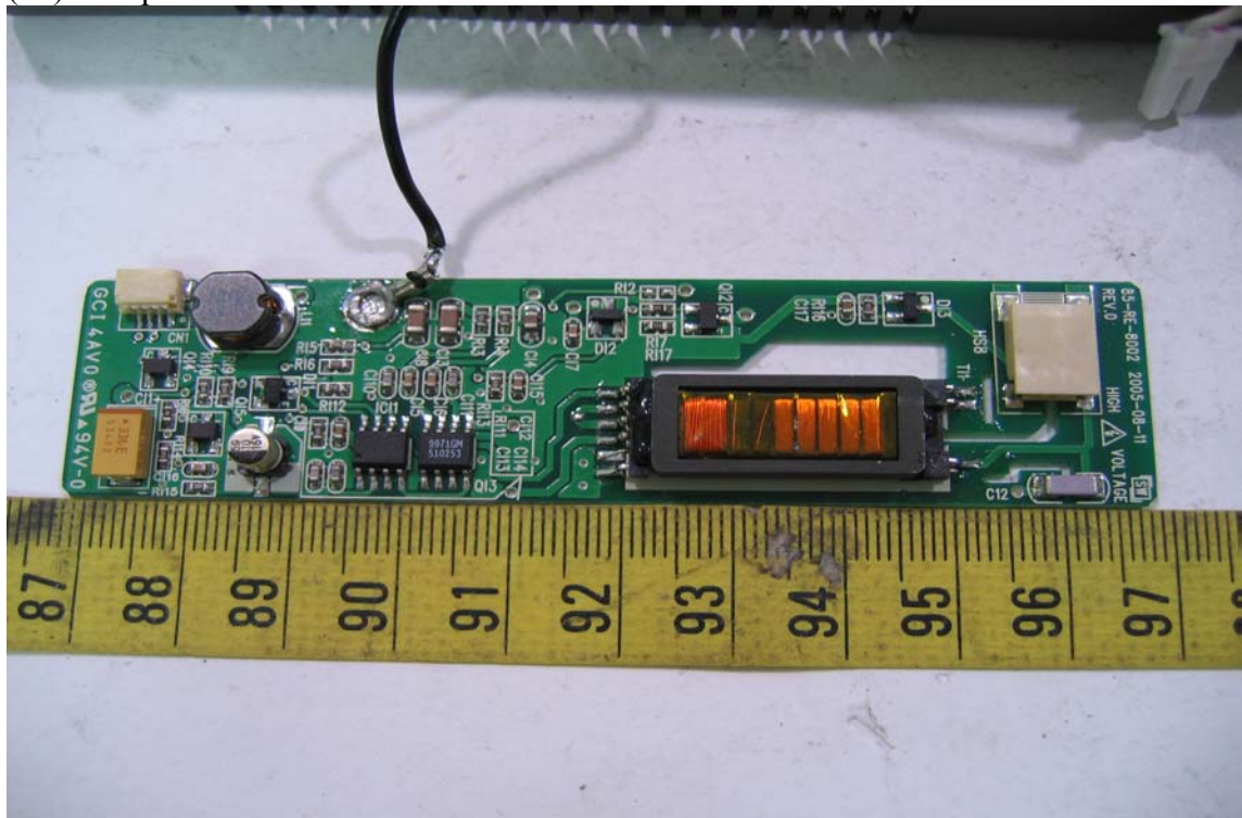
(17) Component View of LCD Panel 's PCB
