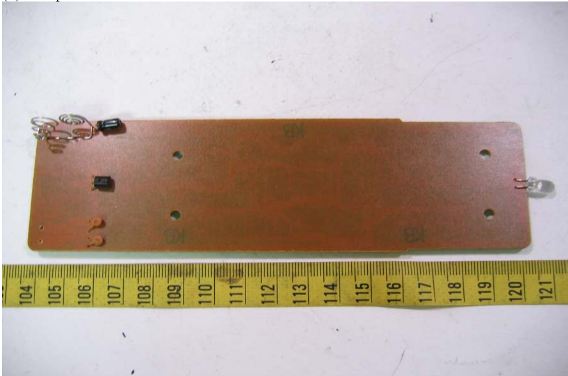
(5) Component View of Remote Controller's PCB
