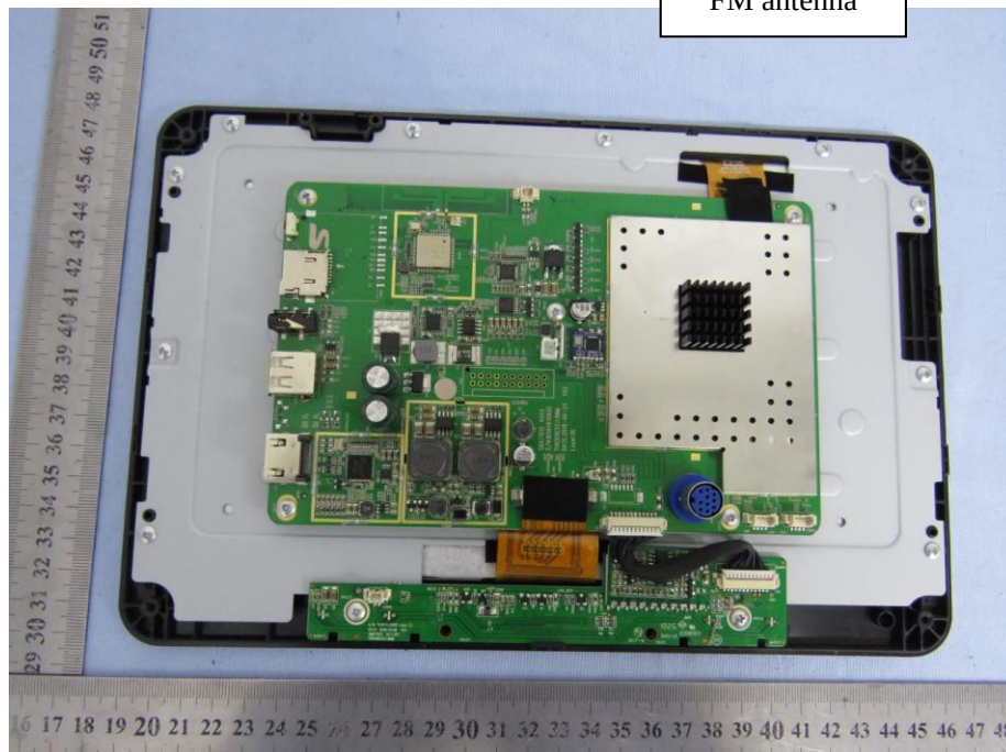
FM antenna
