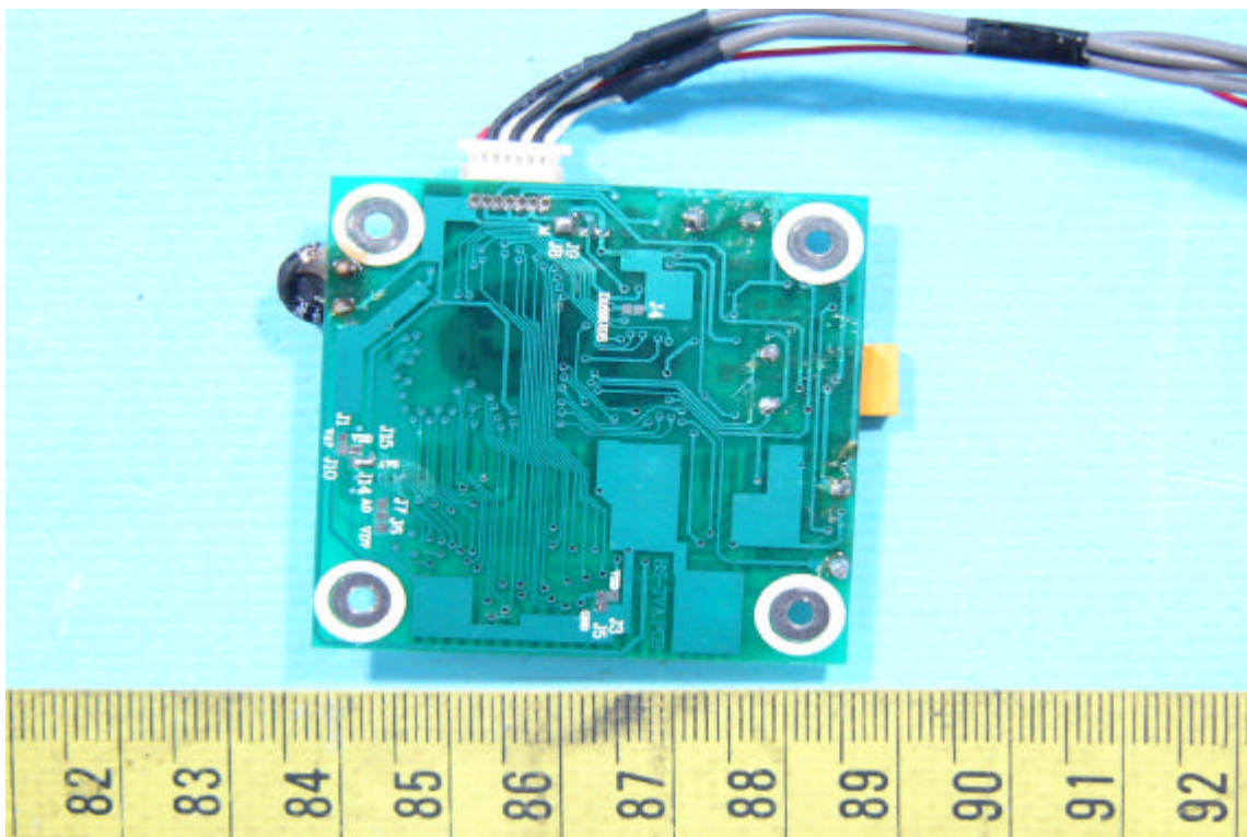
Solder View of the Main PCB
