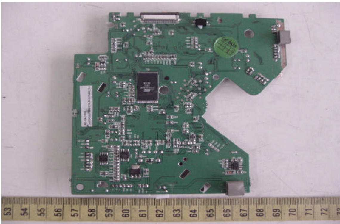
Solder View of PCB 5
