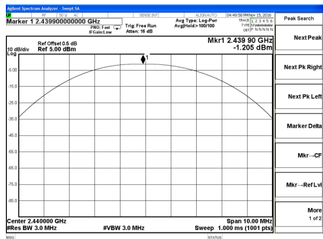
Channel 19 / 2440 MHz
