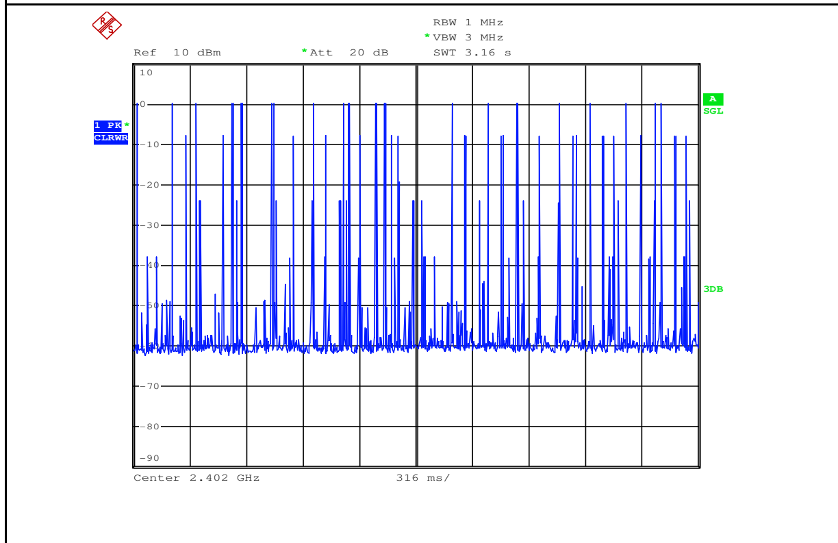
Dwell Time_DH5_2402
