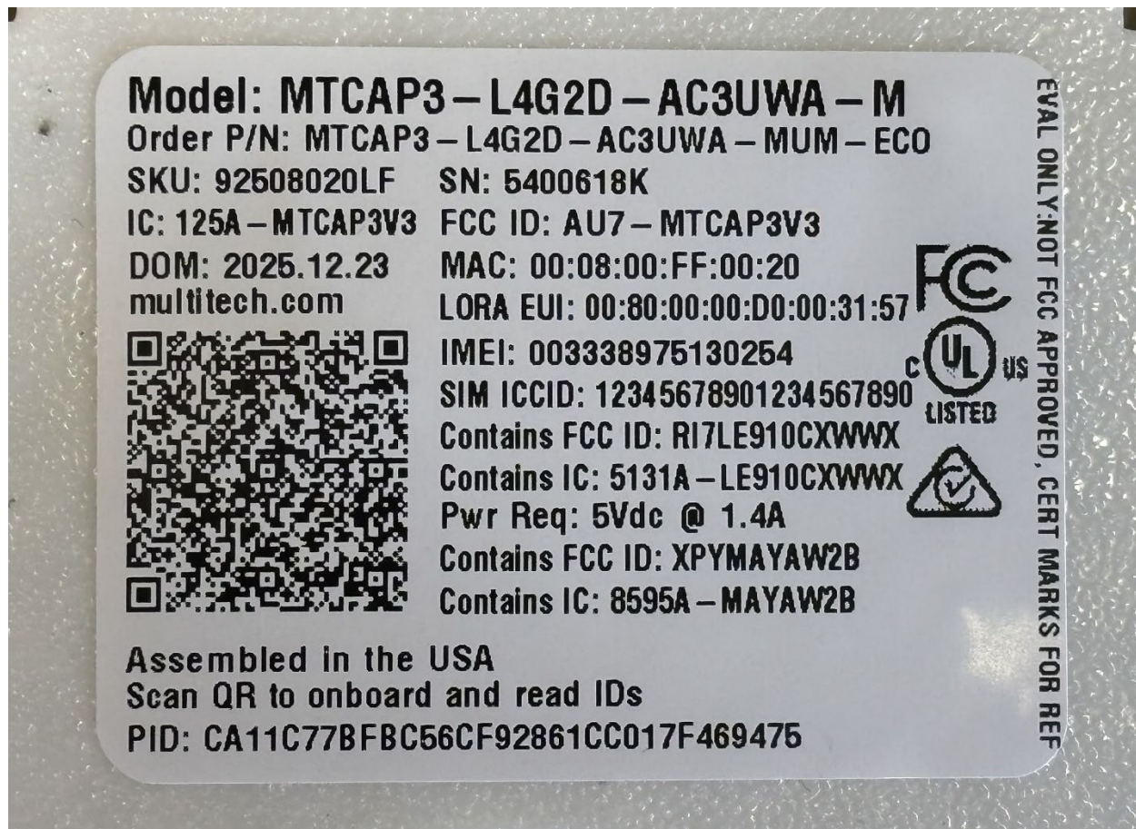
Serial Label on Chassis
