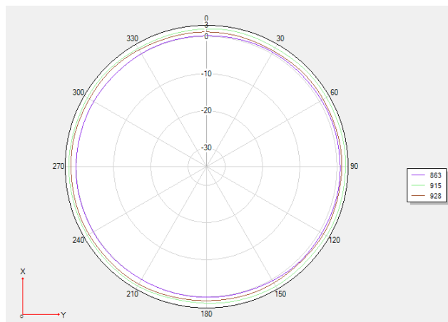
Theta 90 2D
