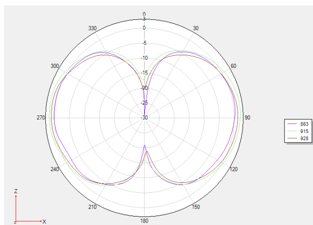
Phi 0 2D
