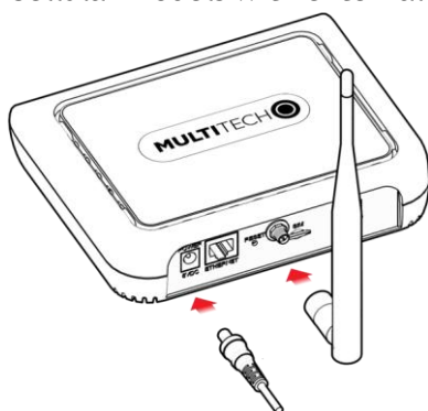
Cellular models with external LoRa antenna
