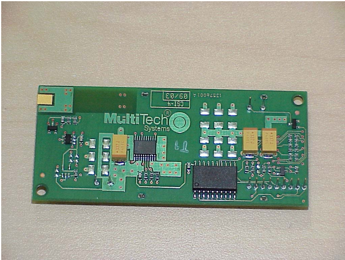
MTSMC-G-F2: Bottom view
