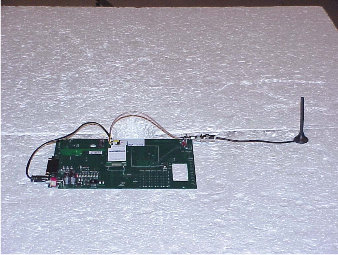
Test setup – Radiated Emissions (MTSMC-G-F2)
