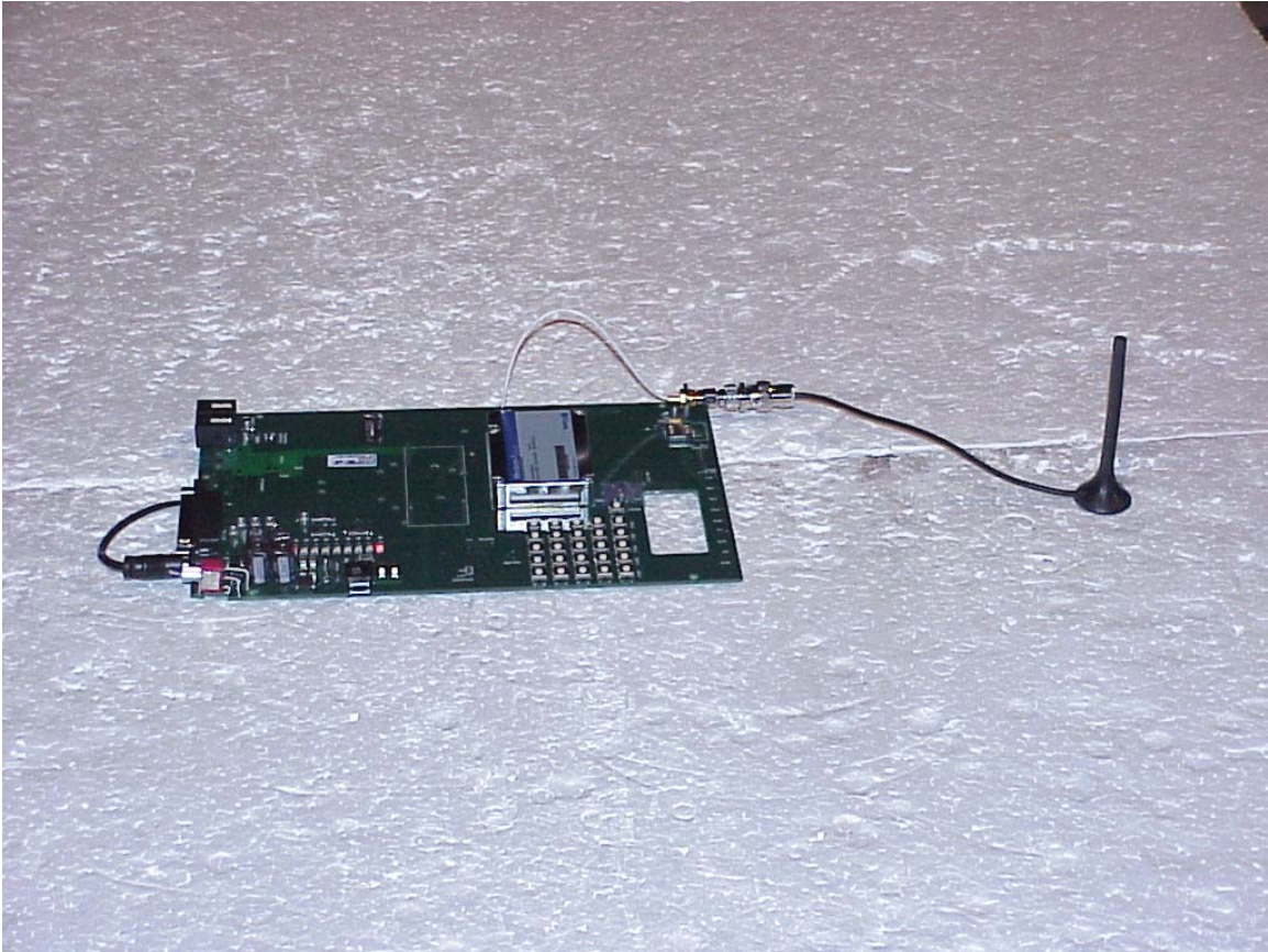
Test setup – Radiated Emissions (MTMMC-G-F2)
