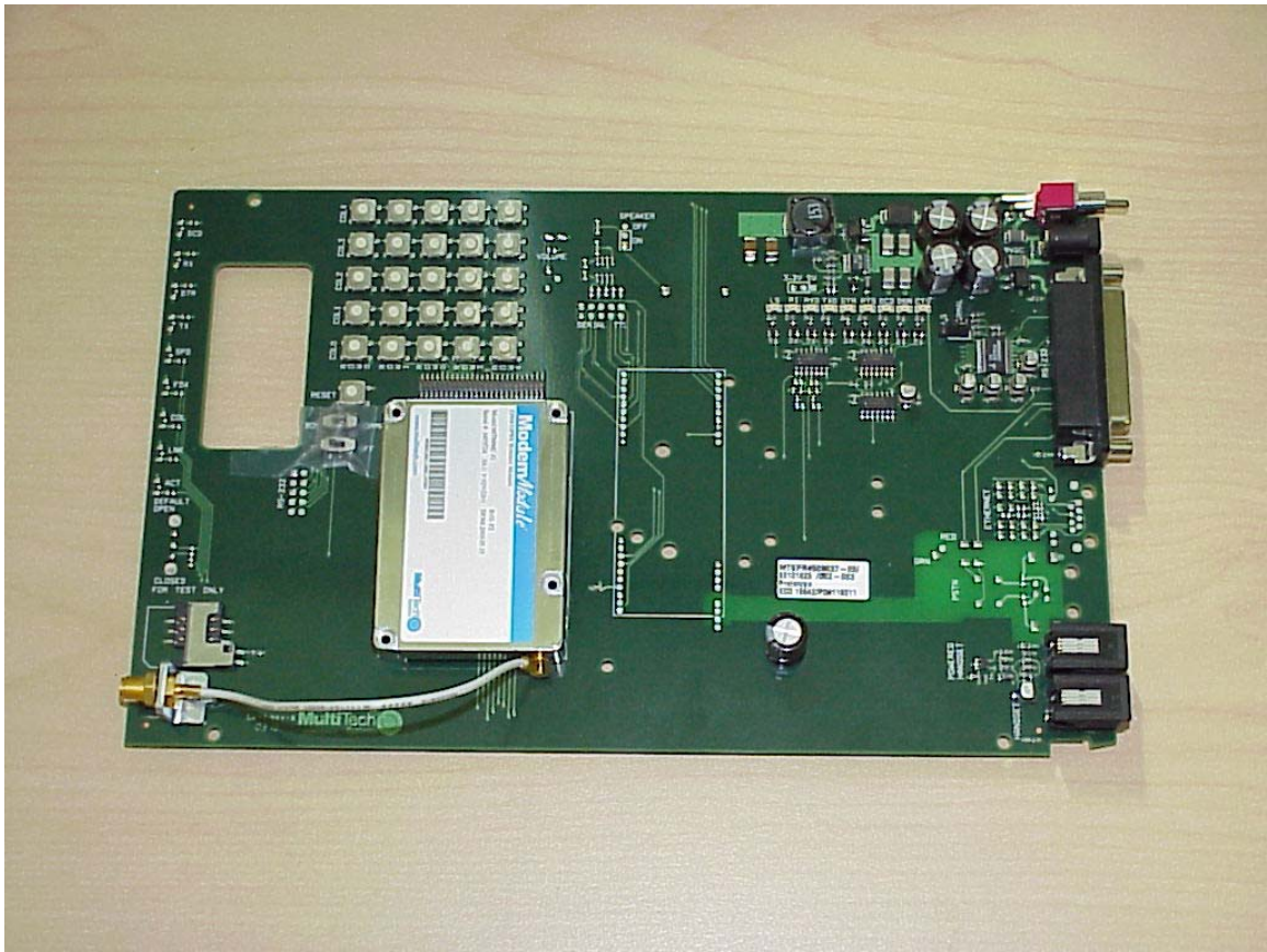
Test fixture for MTMMC-G-F2
