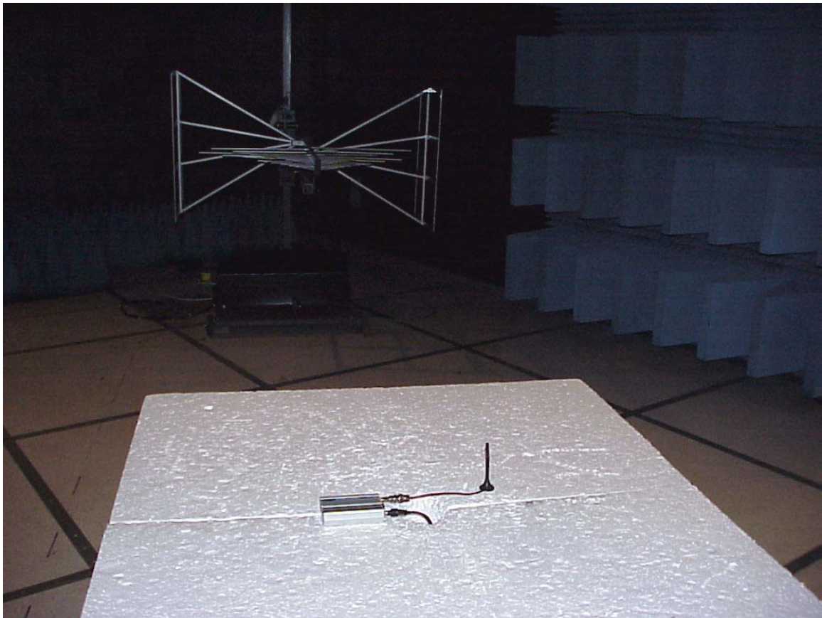
Test setup – Radiated Emissions (MTCBA-G-F2)
