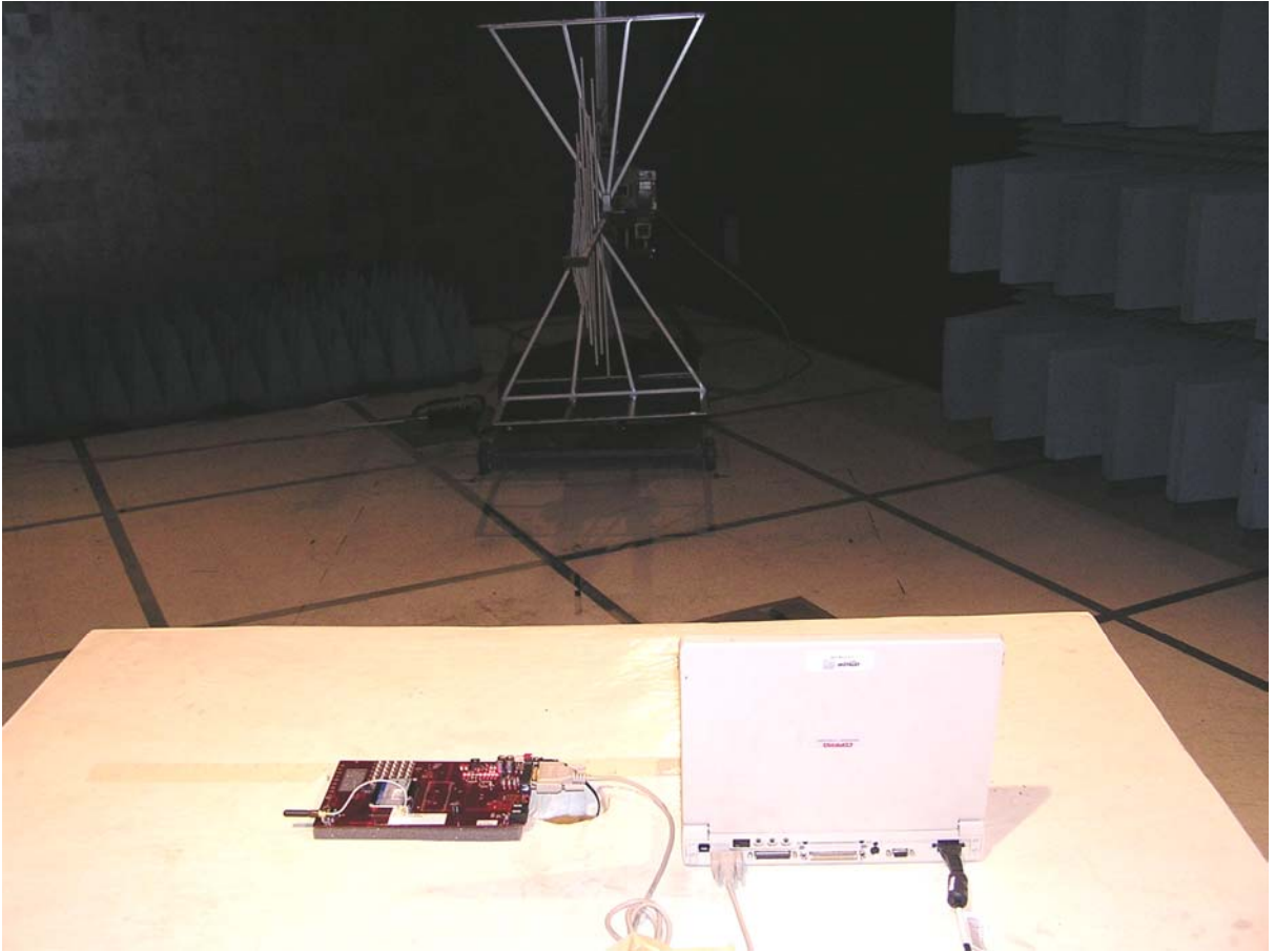
Test setup – Radiated Emissions with Laptop
