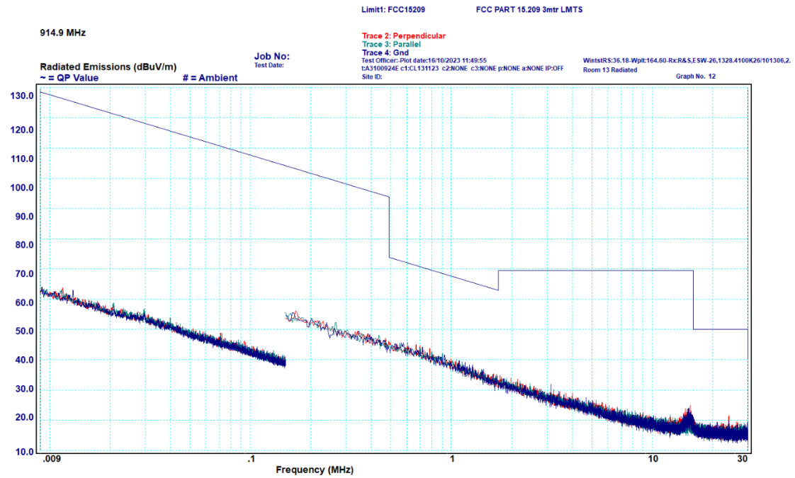
Graph 6-6: Transmitter Spurious Emissions, 9 kHz – 30 MHz, 914.9 MHz
