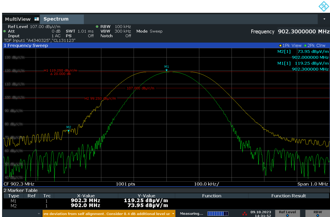
Graph 6-16: Band Edge Emission, Lower Band-edge, 902 MHz
