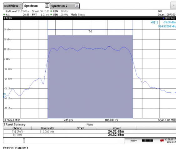
Figure 7.4.2-2: Mid Channel
