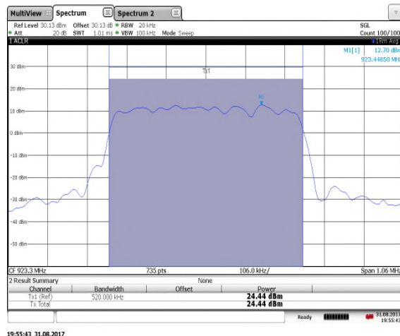
Figure 7.4.2-1: Low Channel
