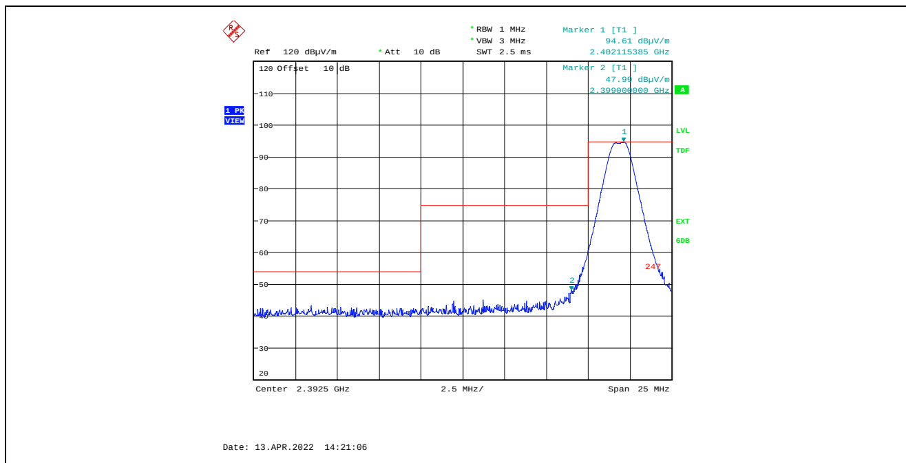
Plot 5.4.4.2.1. Band-Edge RF Radiated Emissions at 3 m, Vertical Polarization 2402 MHz, Low End of Frequency Band
