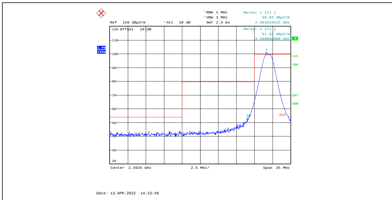
Plot 5.4.4.2.2. Band-Edge RF Radiated Emissions at 3 m, Horizontal Polarization 2402 MHz, Low End of Frequency Band
