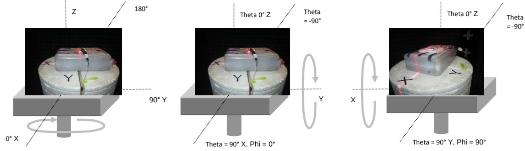
Azimuth Cut (Theta Axis = 90°)
