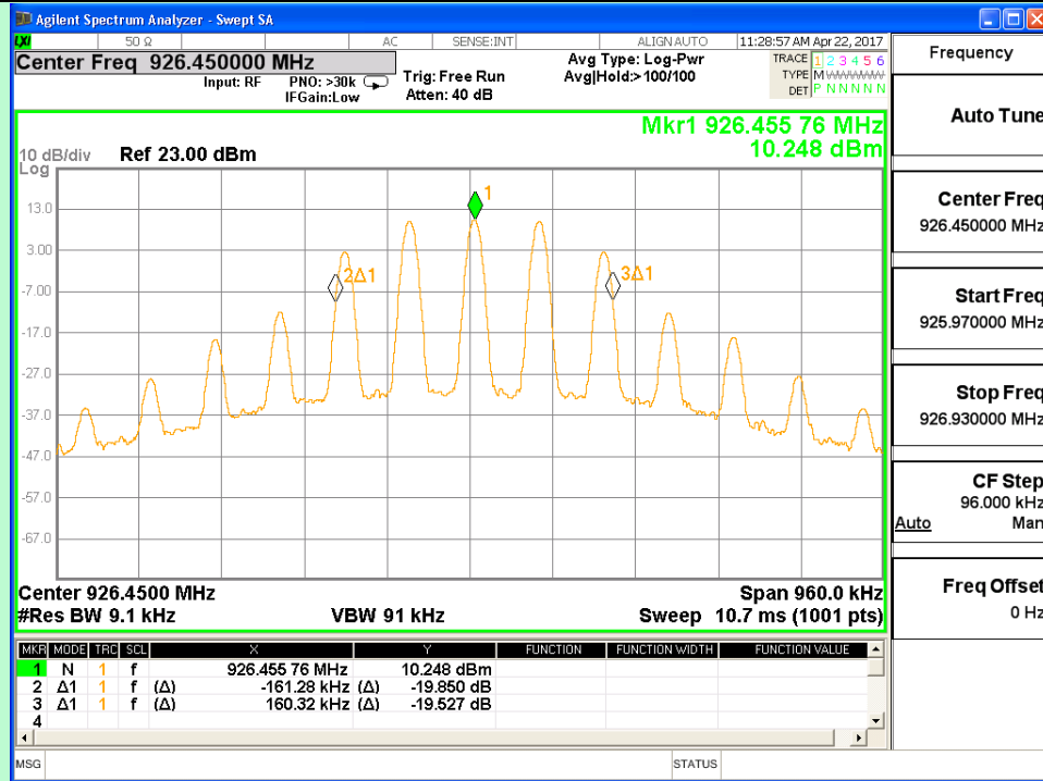
Channel 55 (926.45MHz)
