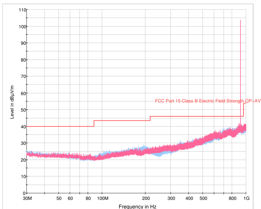
Antenna-1, Channel 28 (916 MHz)
