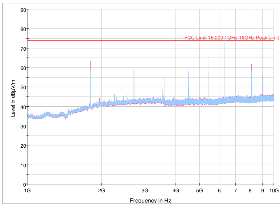
Antenna-3, Channel 1 (903.55 MHz)
