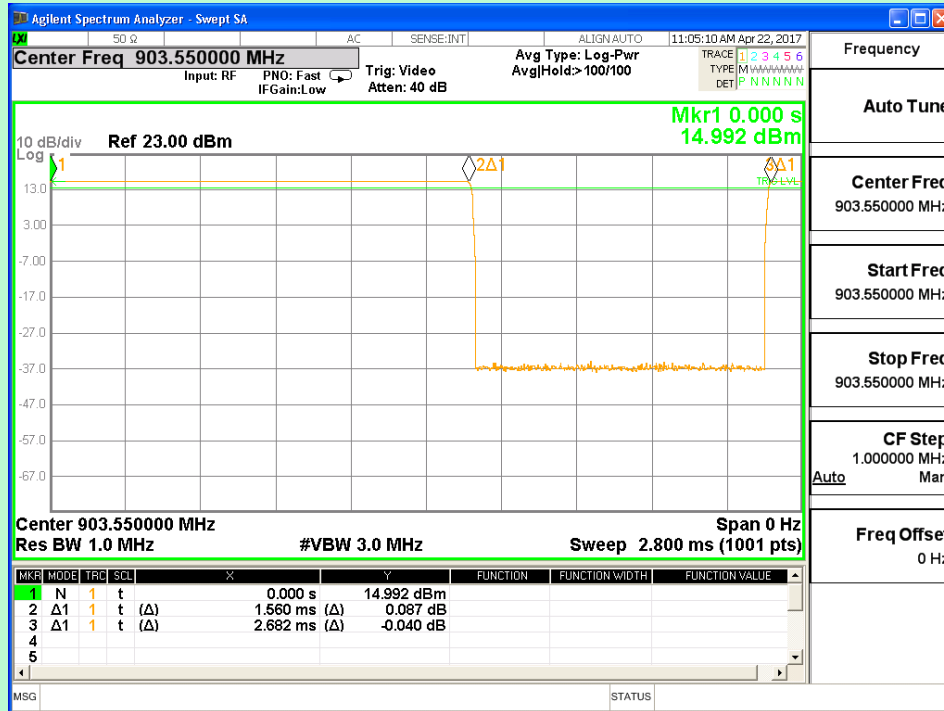
Channel 1 (903.55 MHz)
