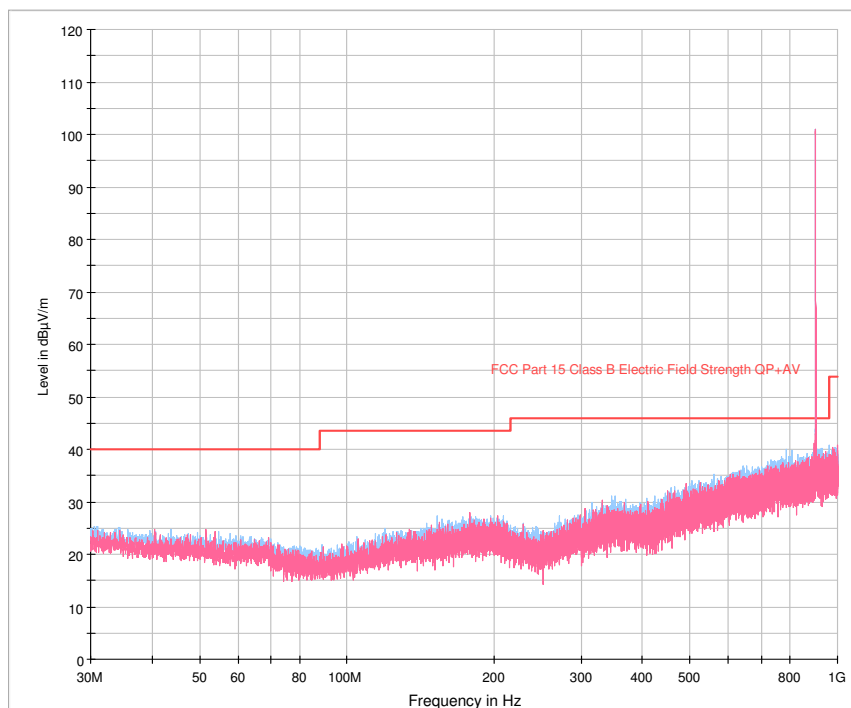
Antenna-2, Channel 1 (903.55 MHz)
