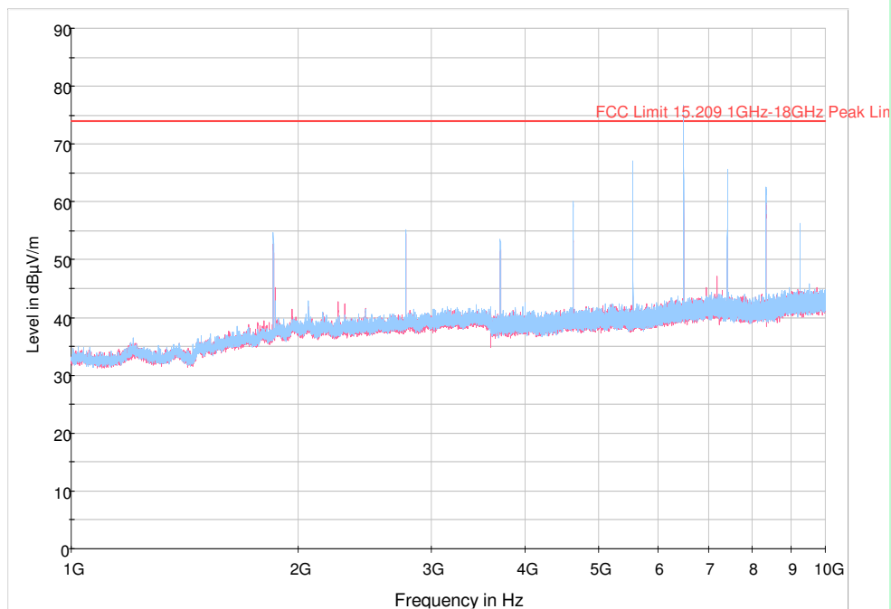
Antenna-1, Channel 55 (926.45 MHz)
