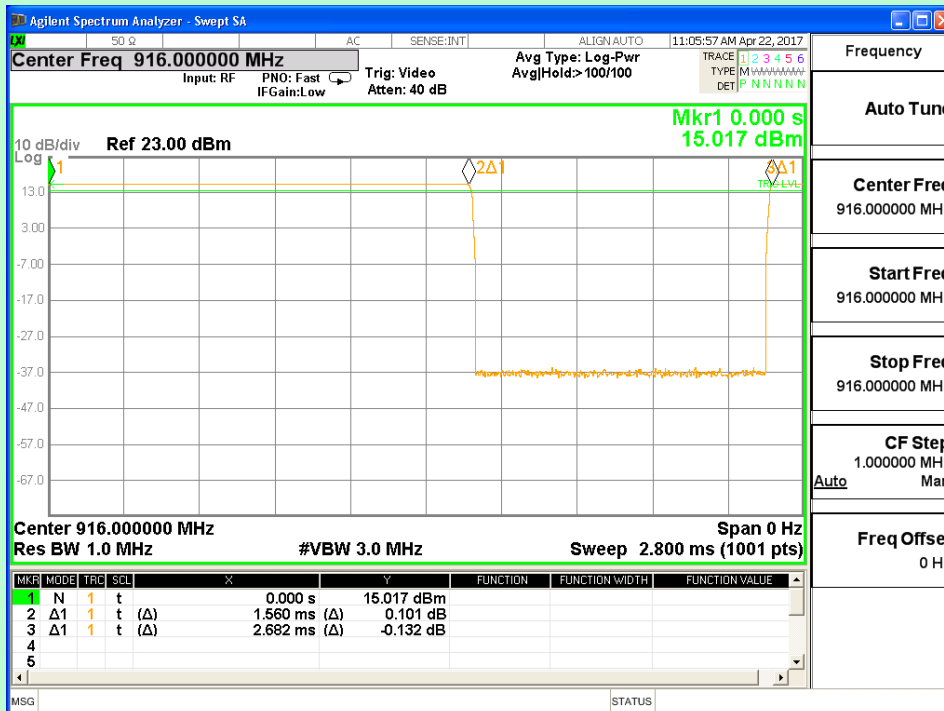
Channel 28 (916MHz)
