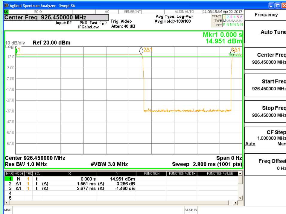
Channel 55 (926.45 MHz)
