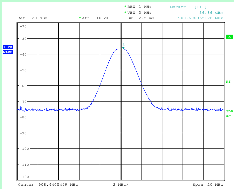
Antenna-3, Channel 2 (908.425 MHz)
