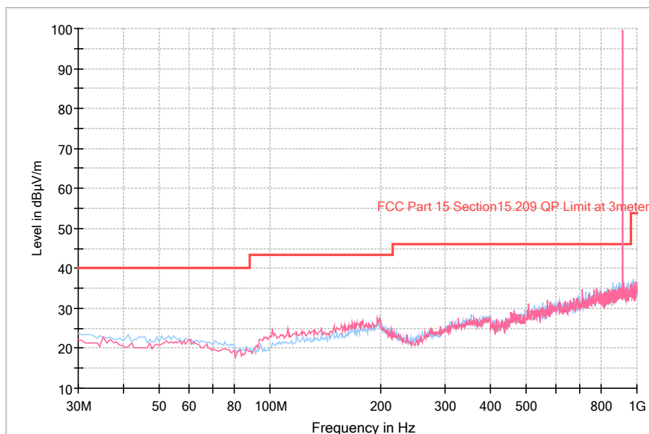
Channel 27 (916.35 MHz)
