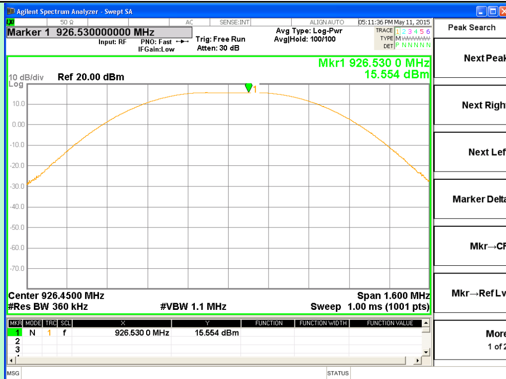
Channel 52 (926.45)
