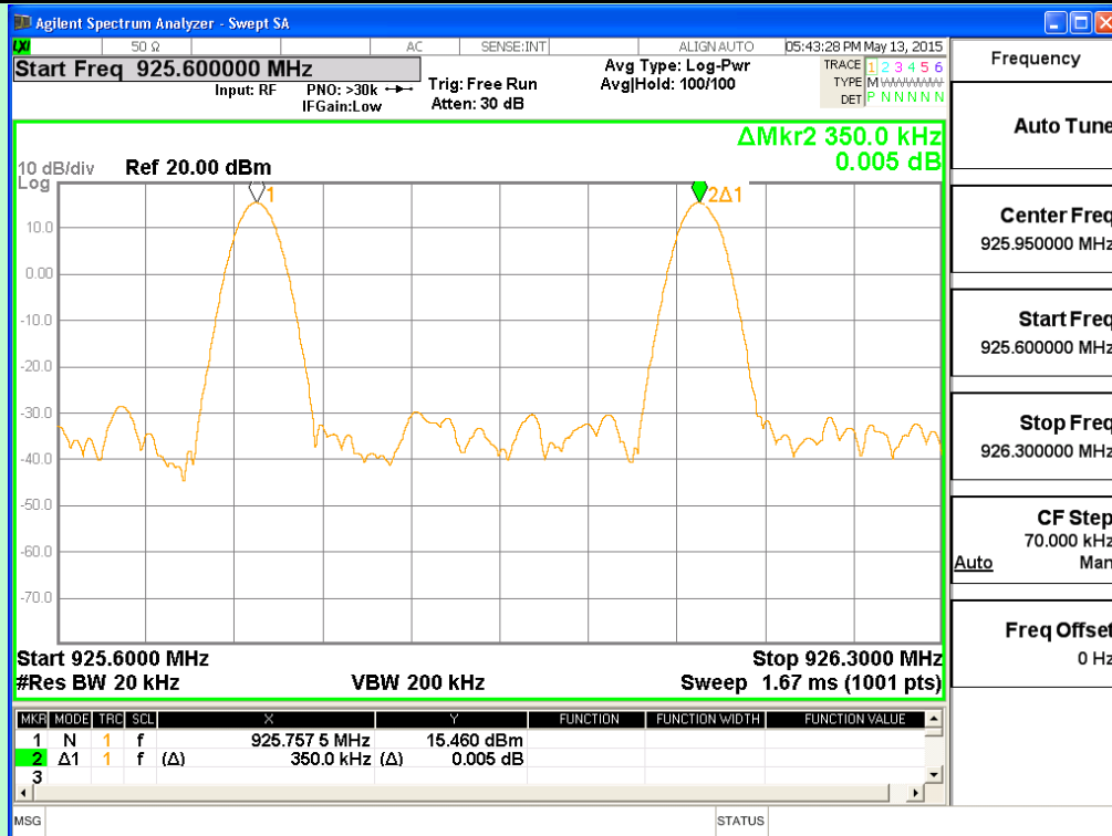
Channel 50 and 51
