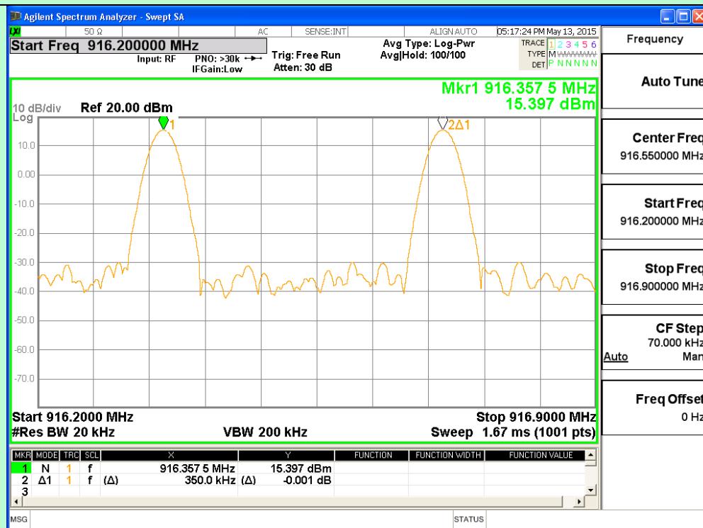
Channel 27 and 28
