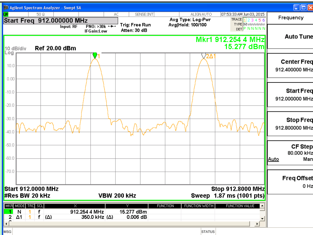
Channel 22 and 23
