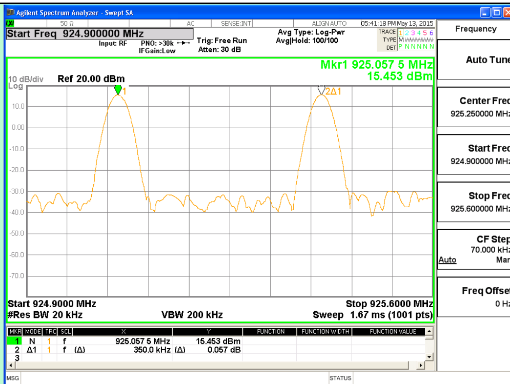
Channel 48 and 49
