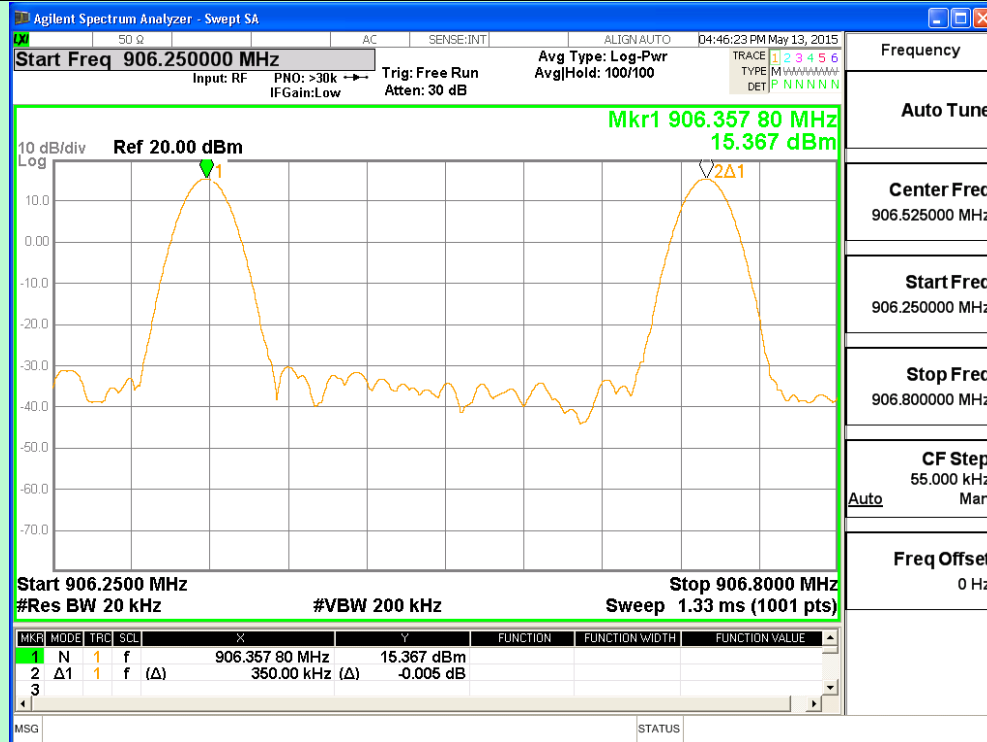
Channel 9 and 10
