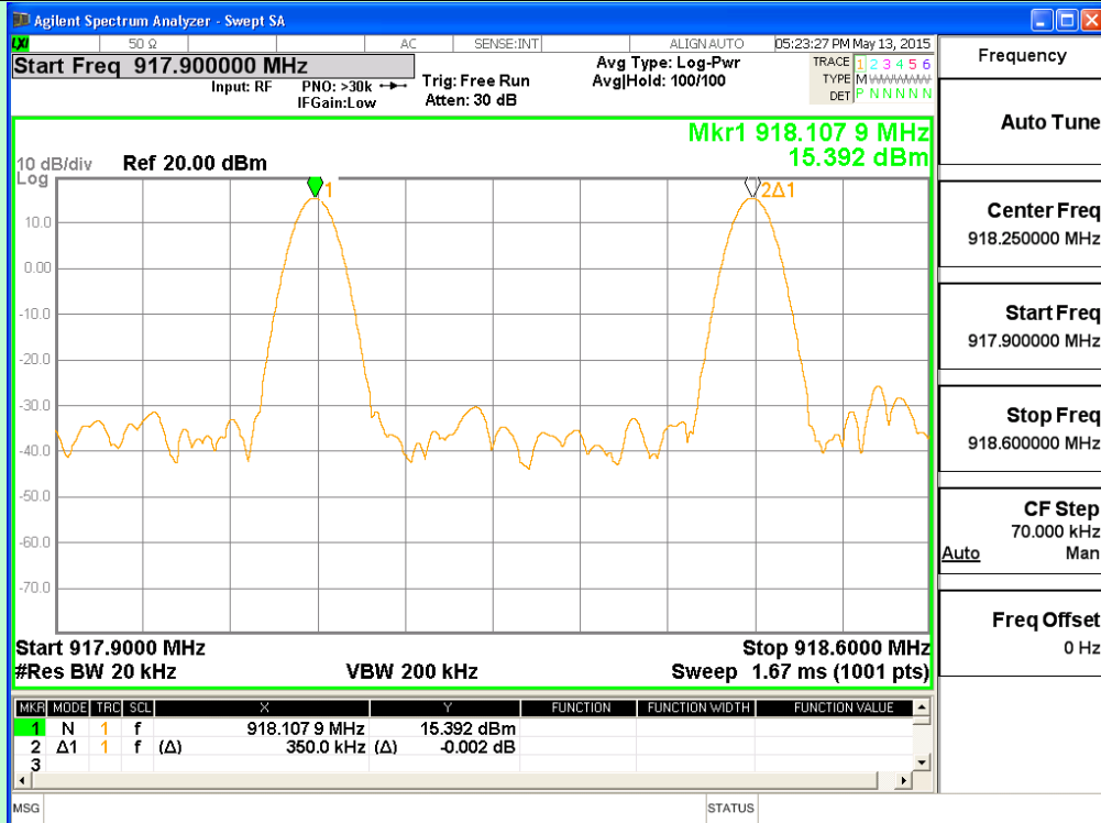
Channel 32 and 33
