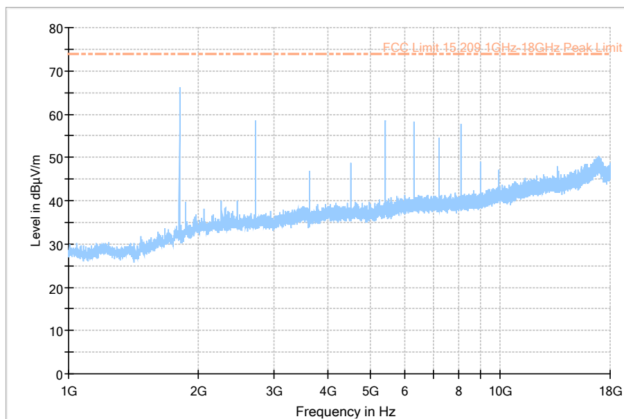
Channel 1 (903.55 MHz)
