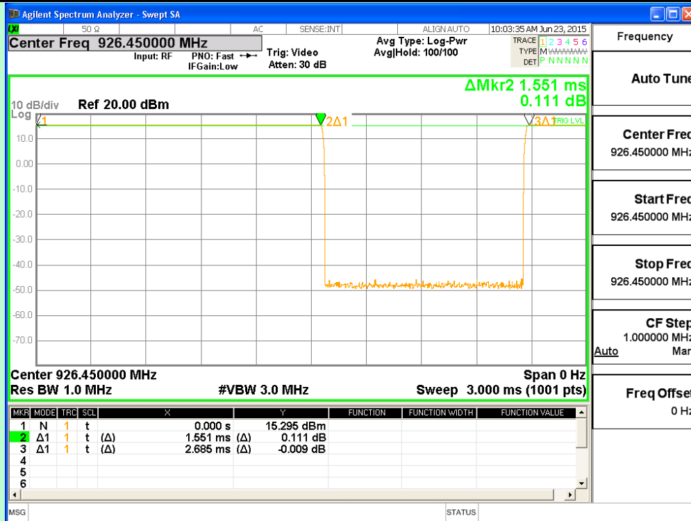
Channel 52 (926.45MHz)
