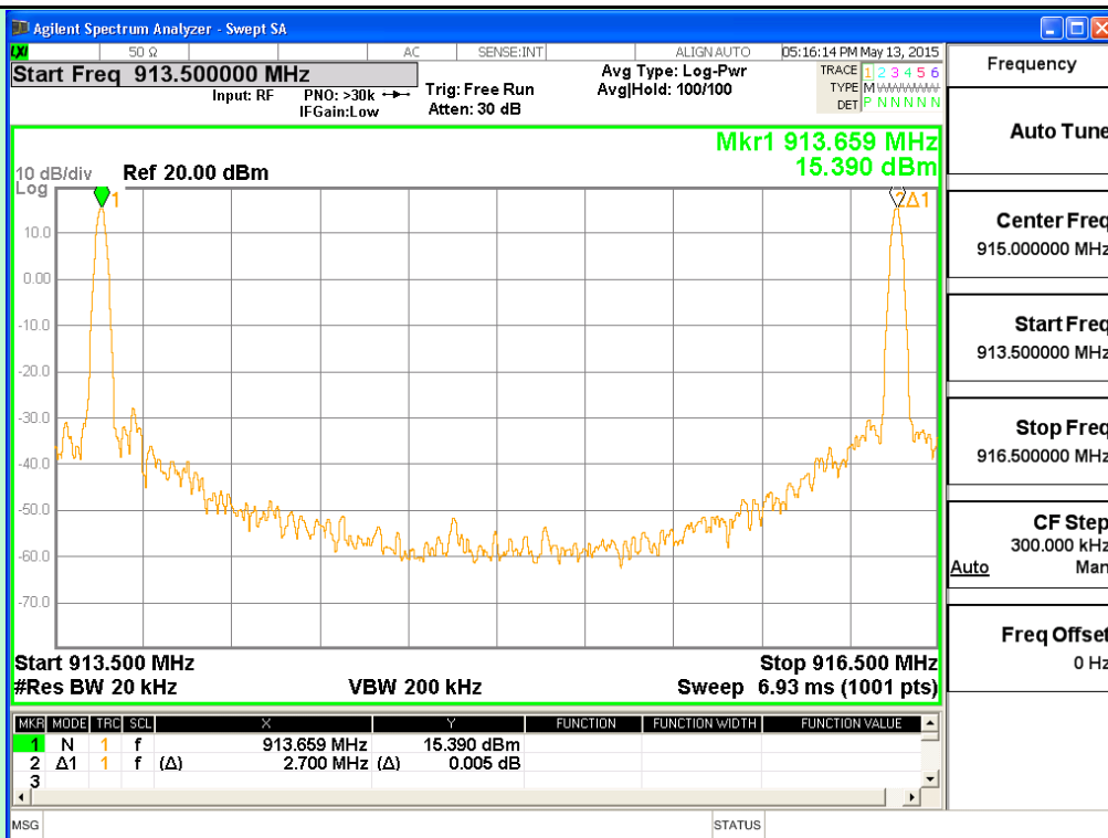
Channel 26 and 27
