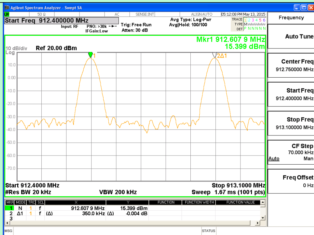
Channel 23 and 24
