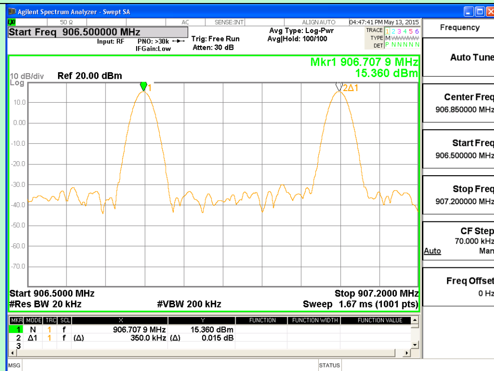
Channel 10 and 11
