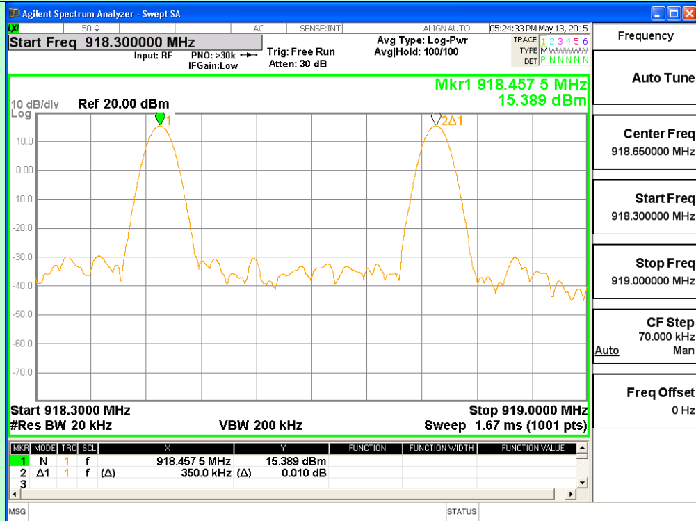
Channel 33 and 34
