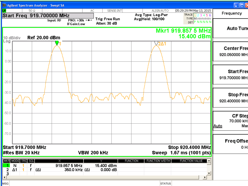
Channel 37 and 38
