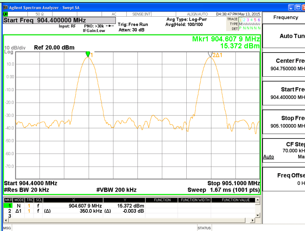
Channel 4 and 5
