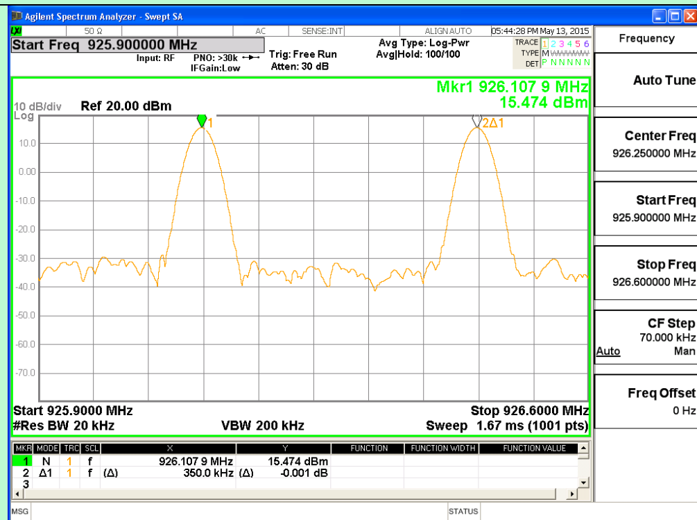
Channel 51 and 52
