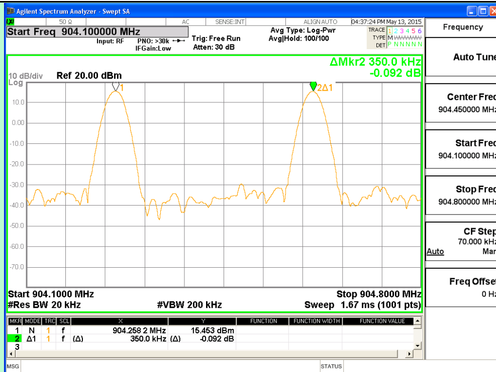
Channel 3 and 4
