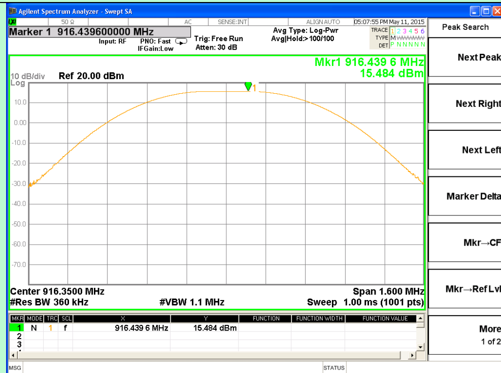
Channel 27 (916.35MHz)
