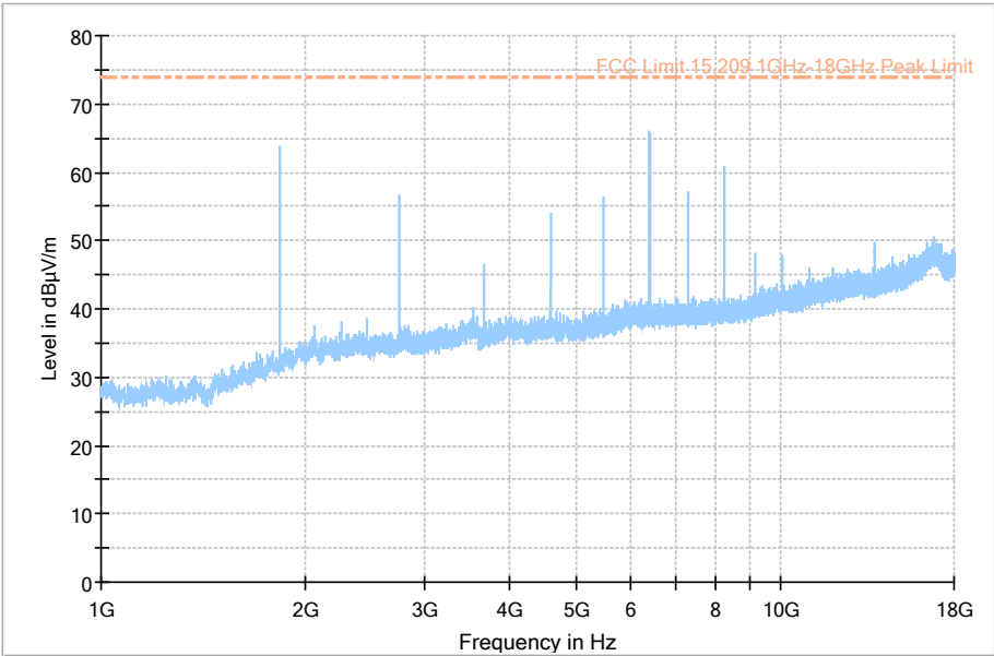
Channel 27 (916.35 MHz)
