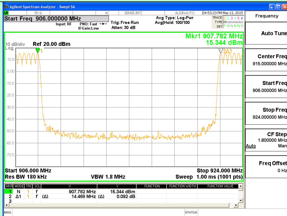
Channel 13 and 40
