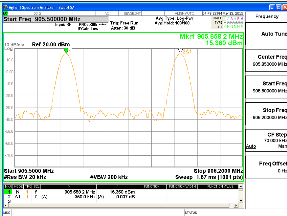
Channel 7 and 8
