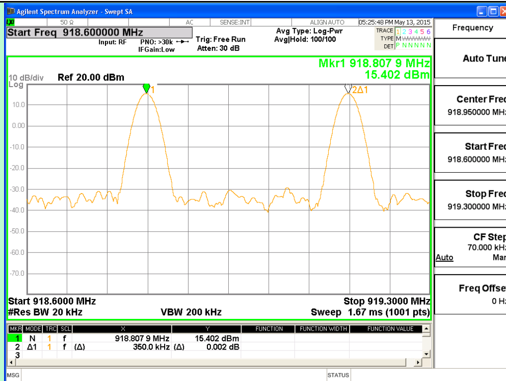
Channel 34 and 35
