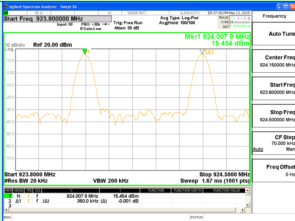
Channel 45 and 46
