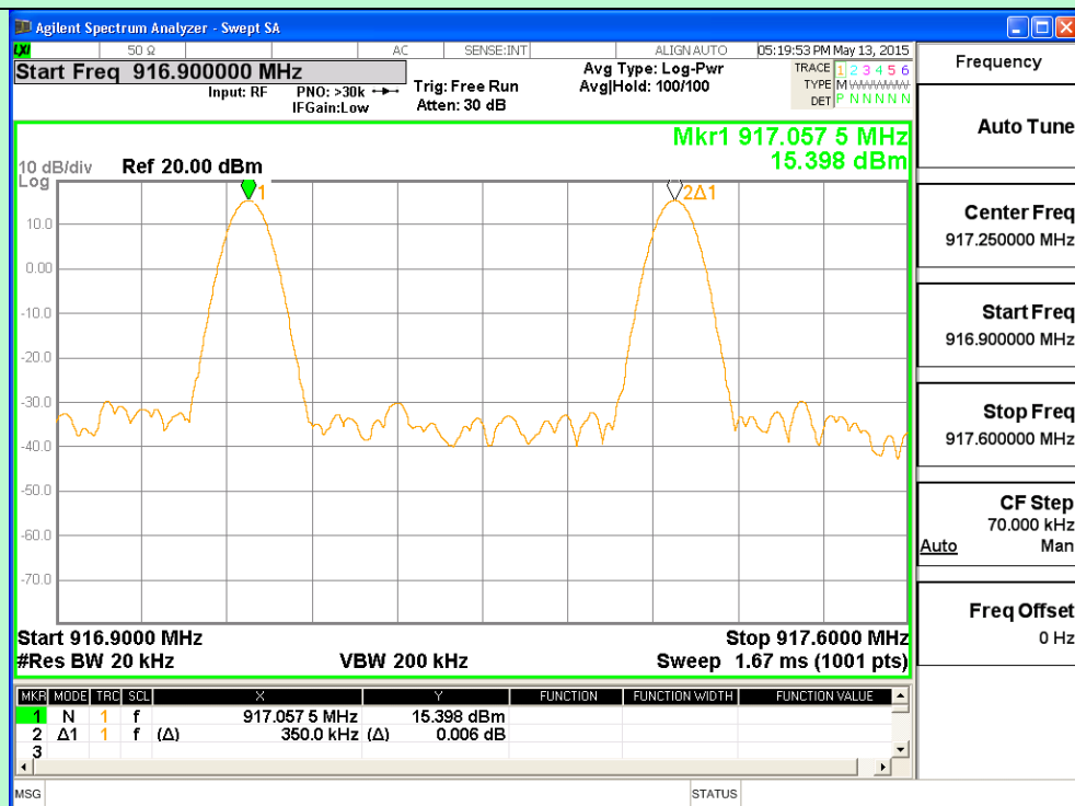
Channel 29 and 30
