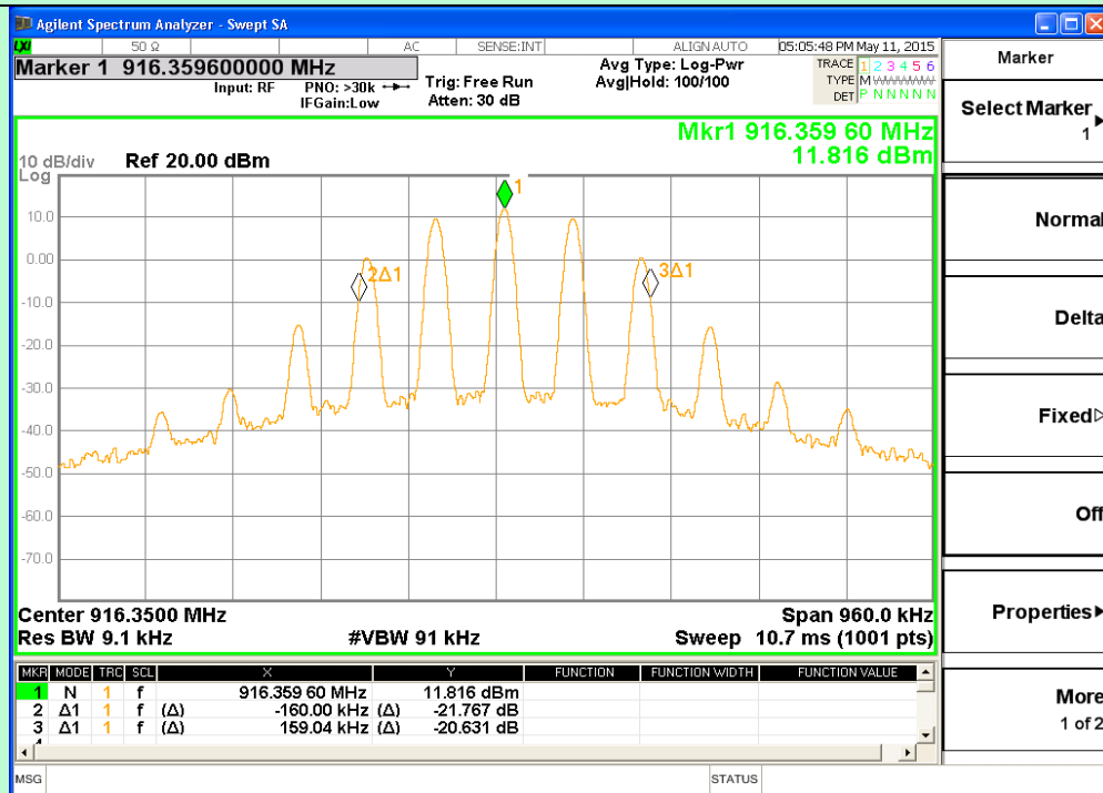
Channel 27 (916.35MHz)
