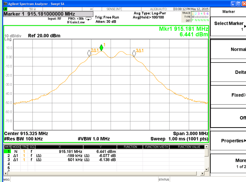
Channel 4 (915.325 MHz)
