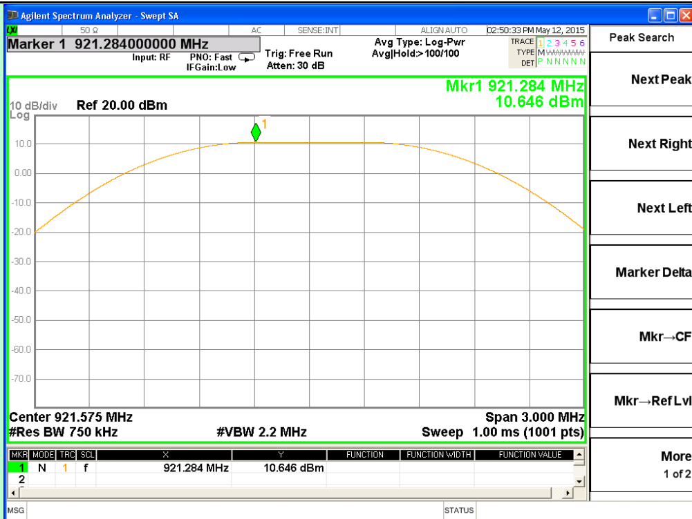
Channel 5 (921.575MHz)
