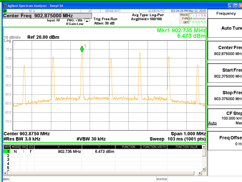
Channel 1 (902.875 MHz)
