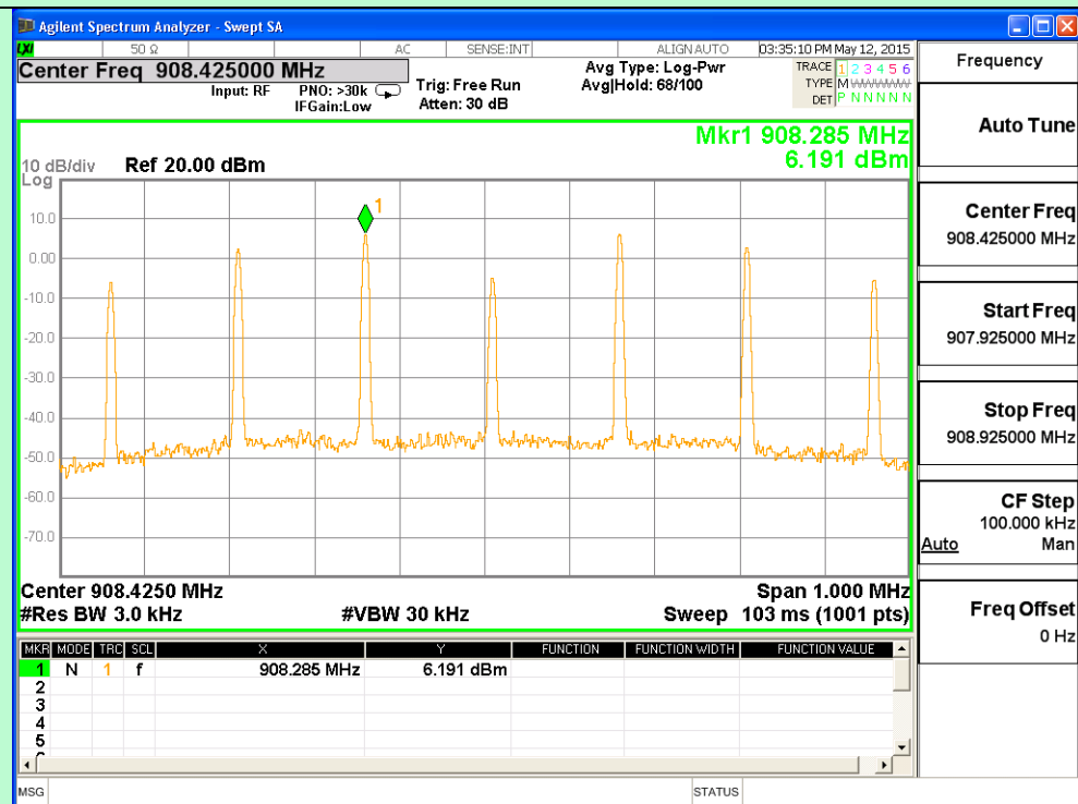
Channel 2 (908.425MHz)
