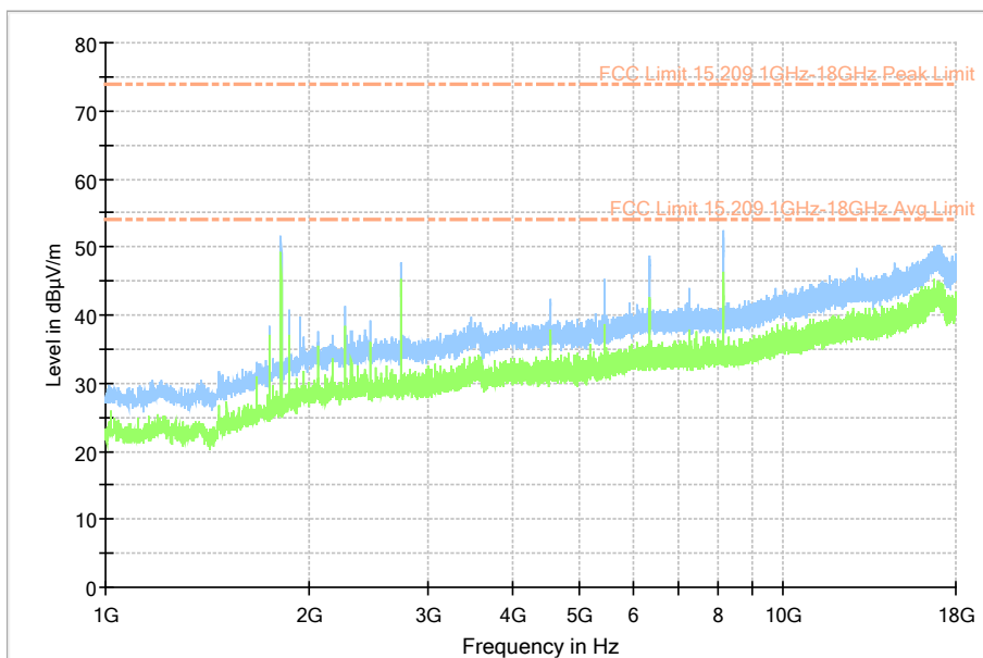
Channel 2 (908.425 MHz)
