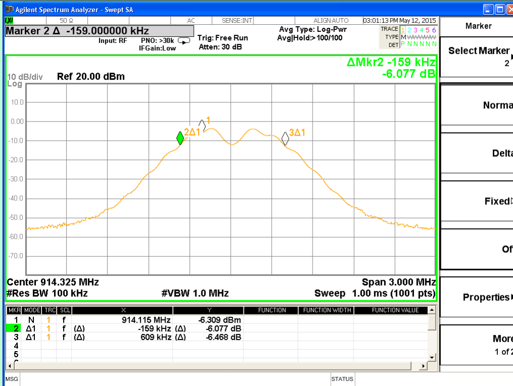
Channel 3 (914.325 MHz)
