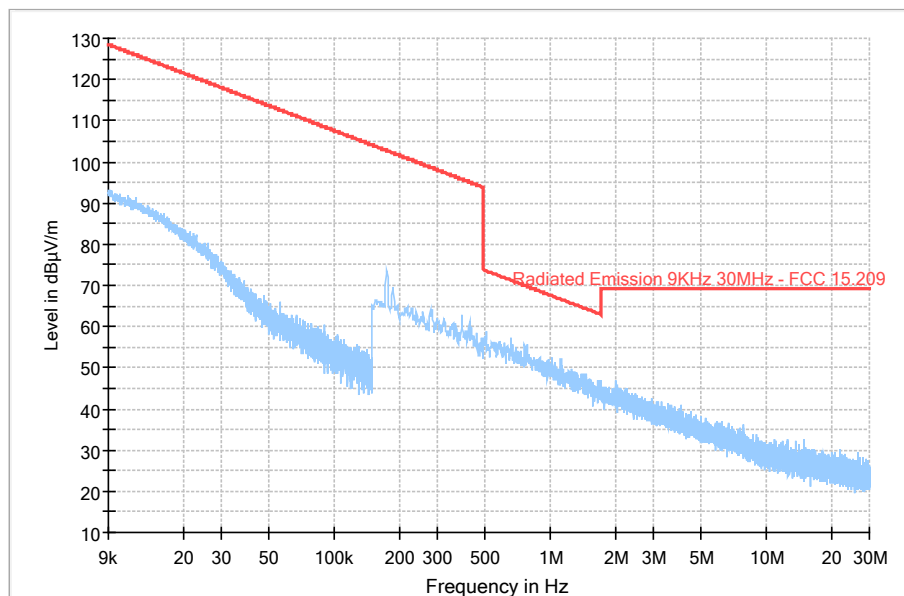
Channel 2 (908.425MHz)
