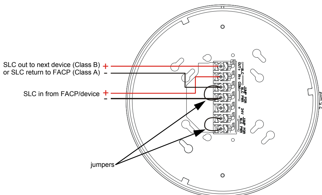
Figure 2.6 Wiring Connections: JFWSG Powered by the SLC
