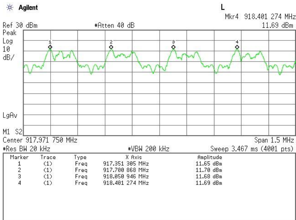
Channel 19-22 (Normal Mode)
