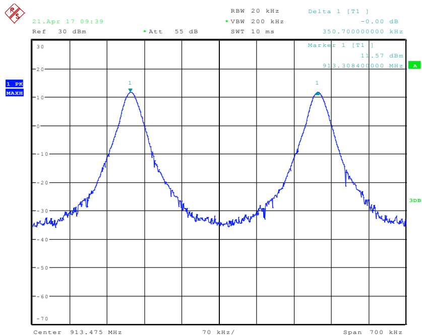
Channel 12 to 13 (Normal)
