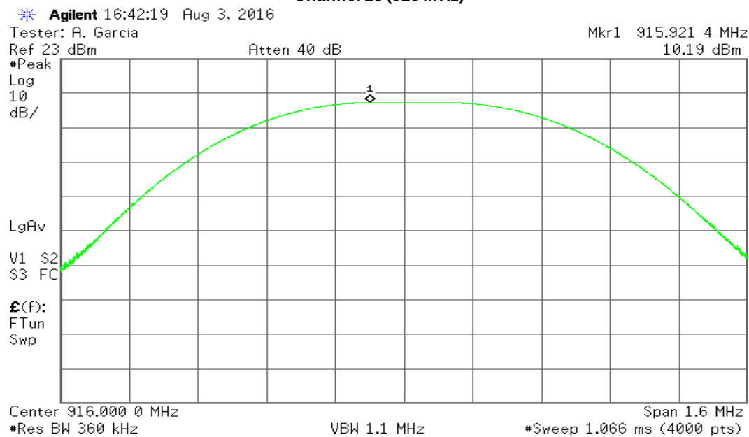
Channel 28 (916 MHz)
