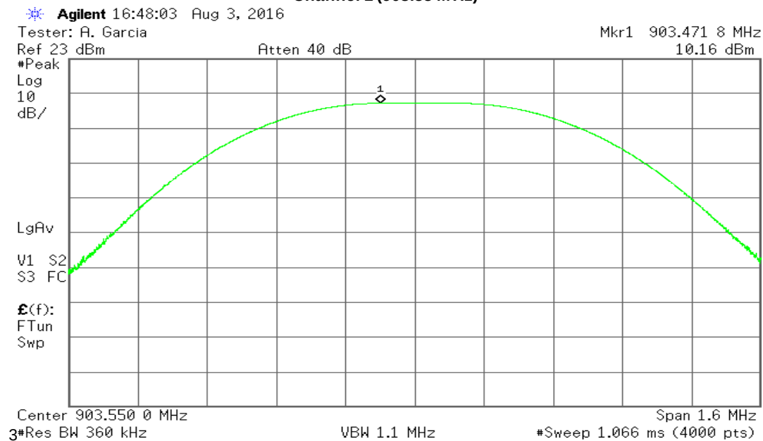
Channel 1 (903.55 MHz)
