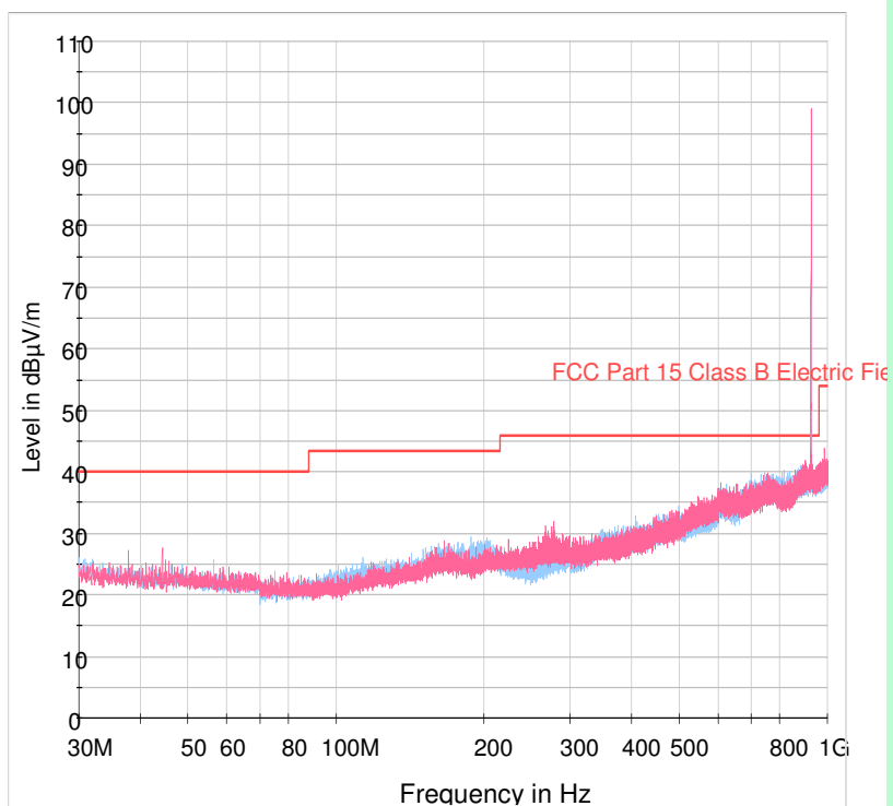
Antenna-1, Channel 55 (926.45 MHz)
