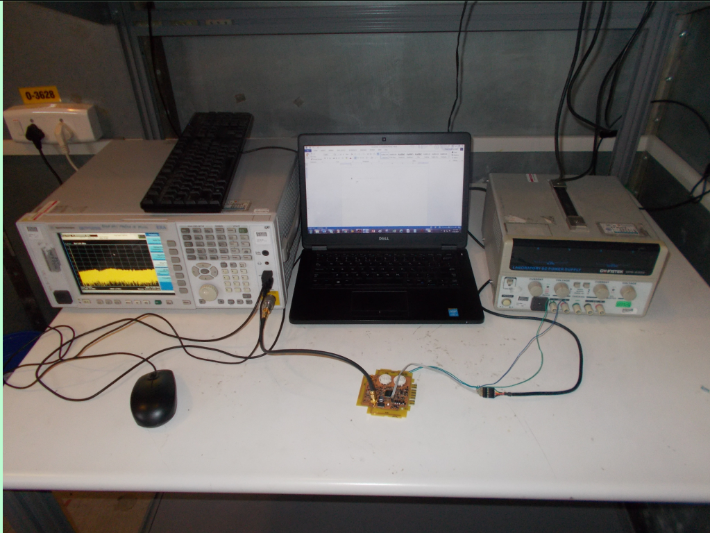
Conducted RF test setup
