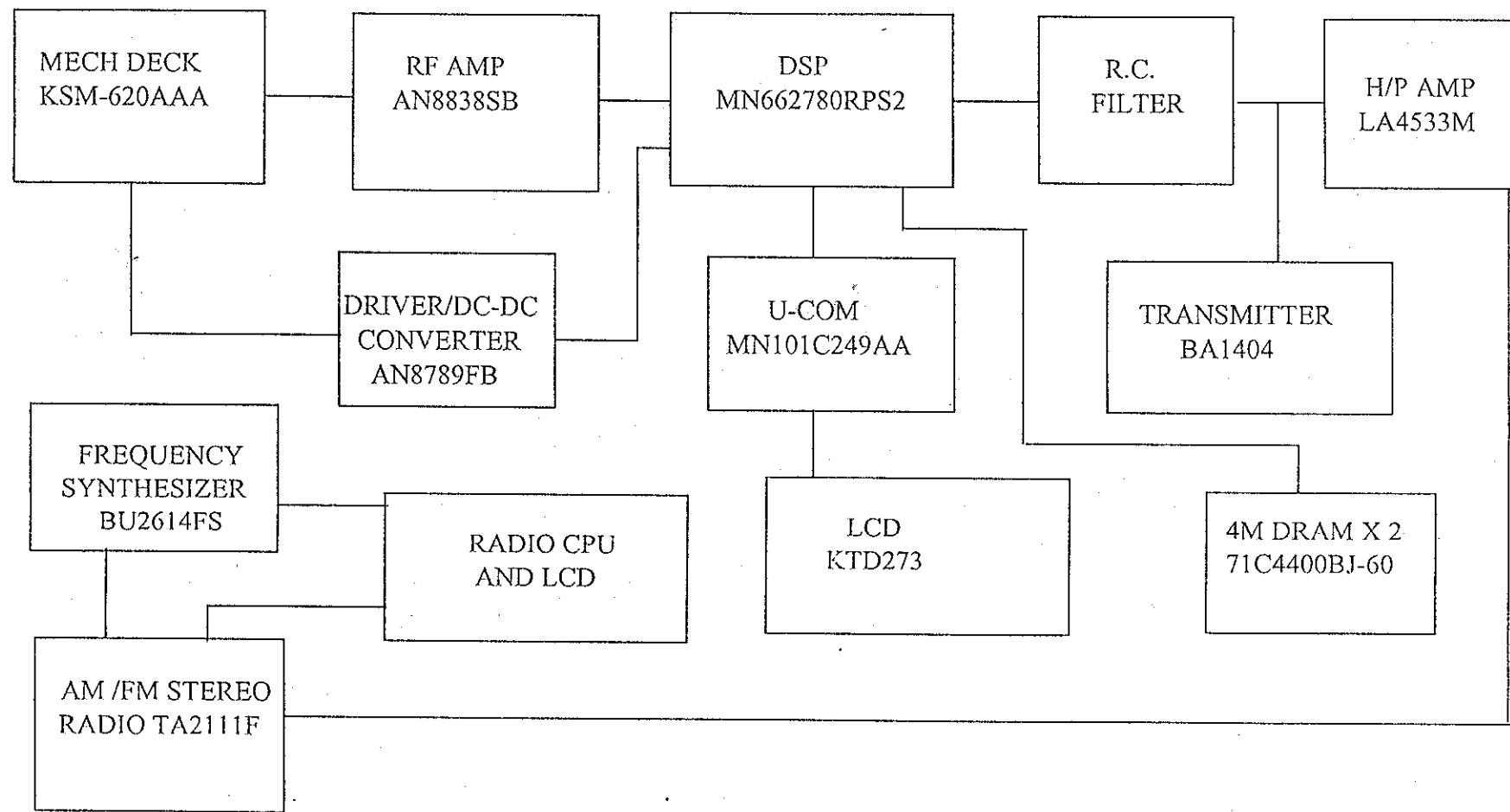
BLOCK DIAGRAM (FOR HD8299C)
