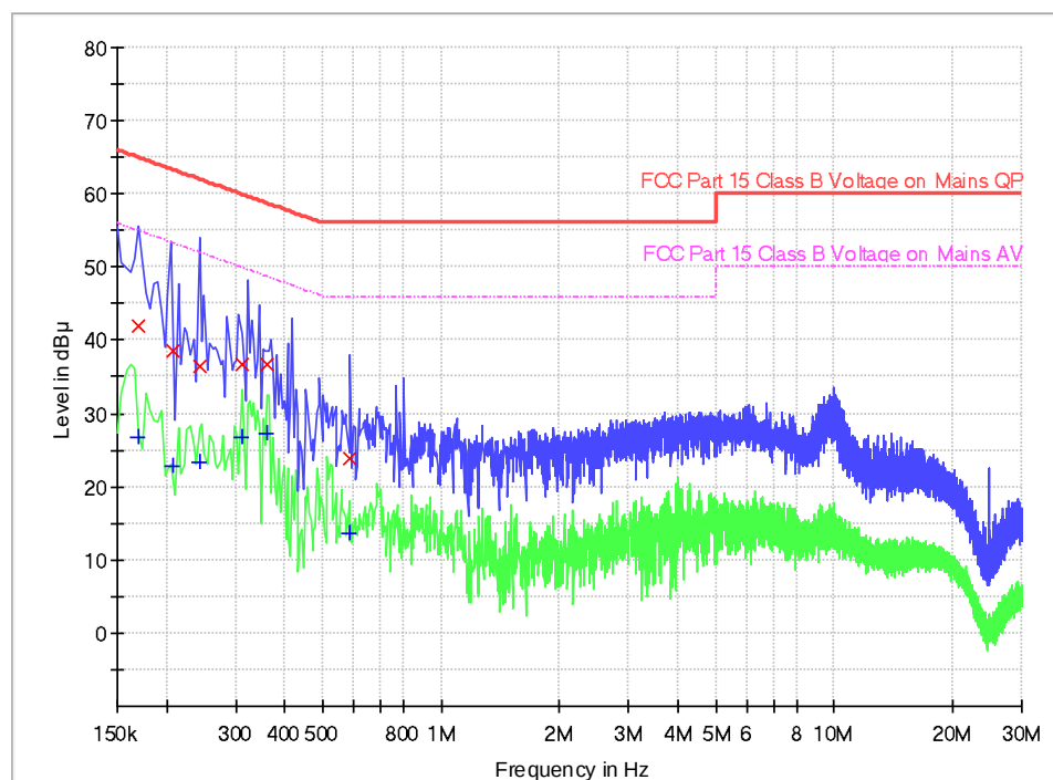
Conducted Emission Test FCC Part 15
