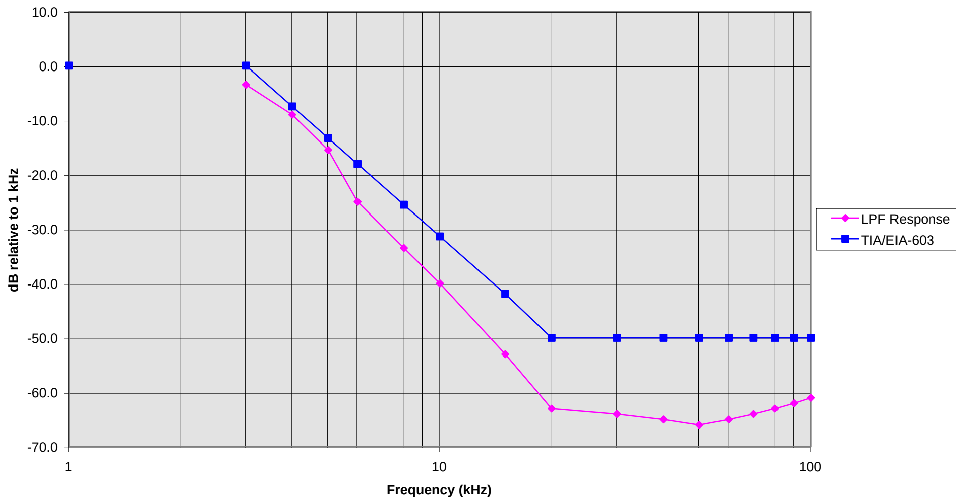
Audio Low Pass Filter Response
