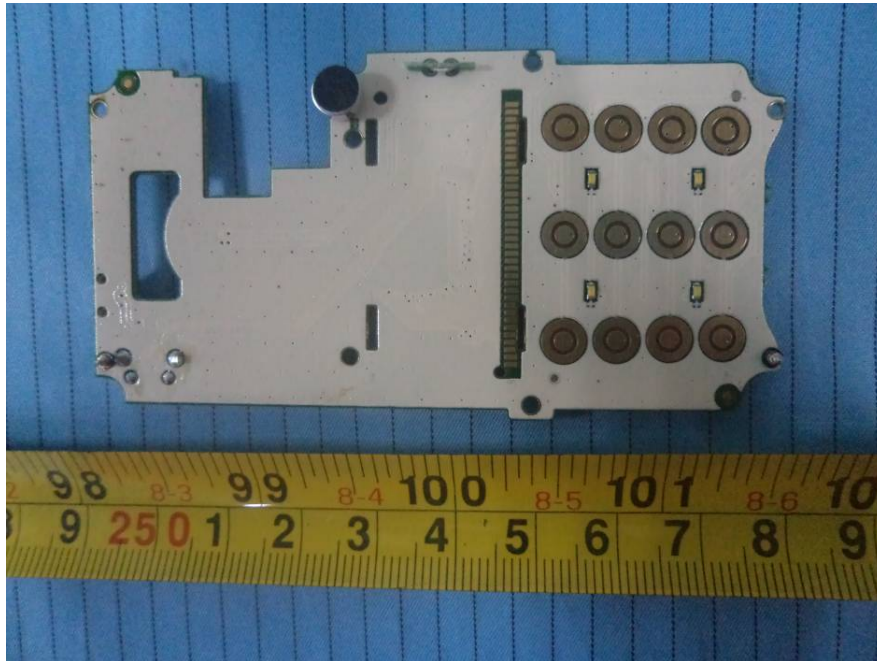
EUT – Main Board 1 Bottom without LCD View
