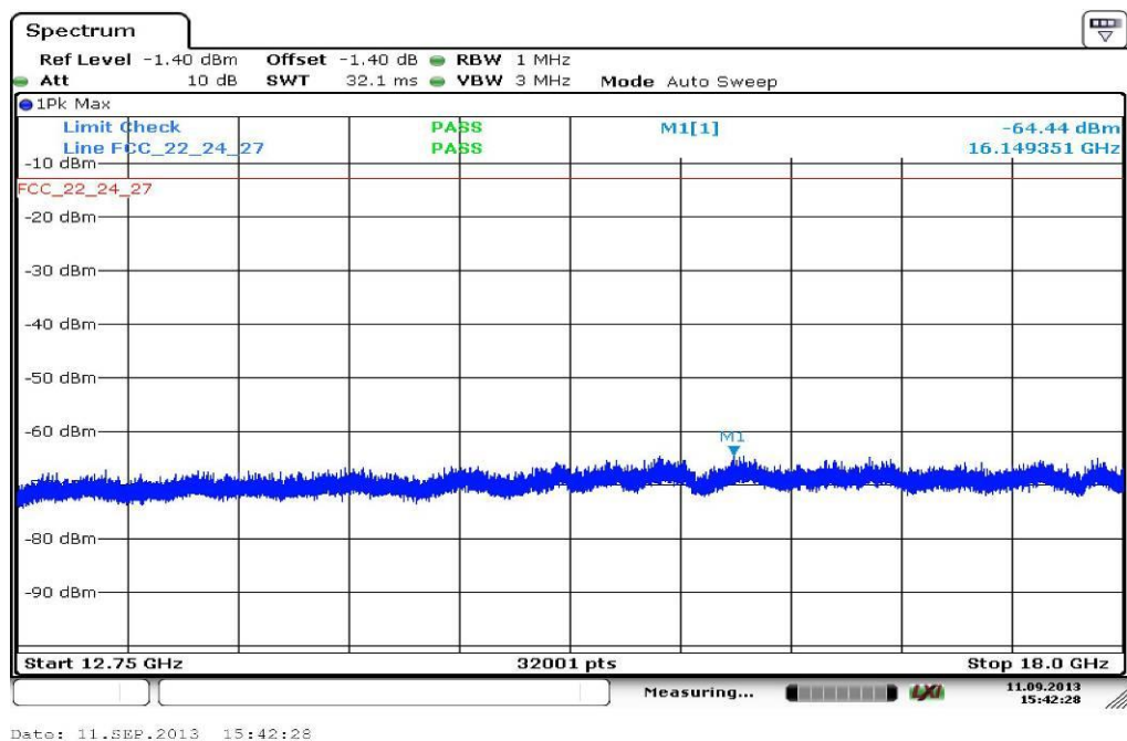
Plot 3: Channel 661 (12.75 GHz - 18 GHz)
