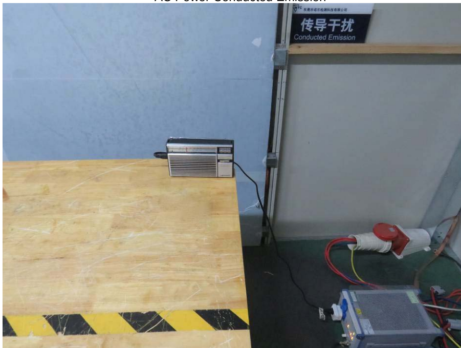
AC Power Conducted Emission
