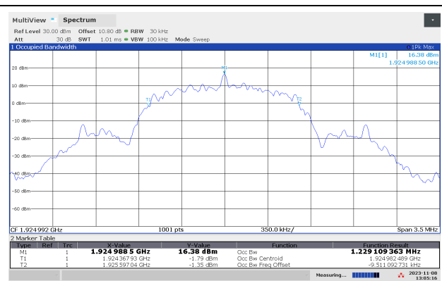
99% Bandwidth, Middle Channel
