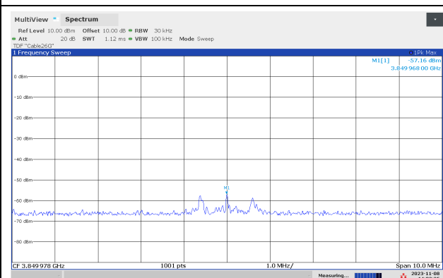
Out-of-Band Emissions 3848 MHz, Middle Channel
