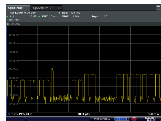
EUT Transmits on Free RECEIVE Slot, BEFORE
