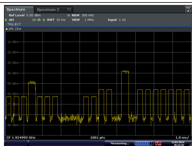
EUT Transmits on Free TRANSMIT Slot, BEFORE
