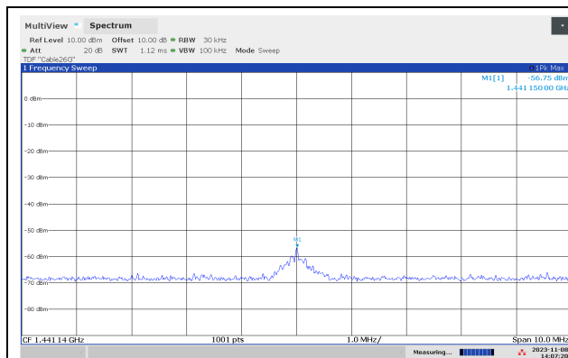
Out-of-Band Emissions 1441 MHz, Lower Channel
