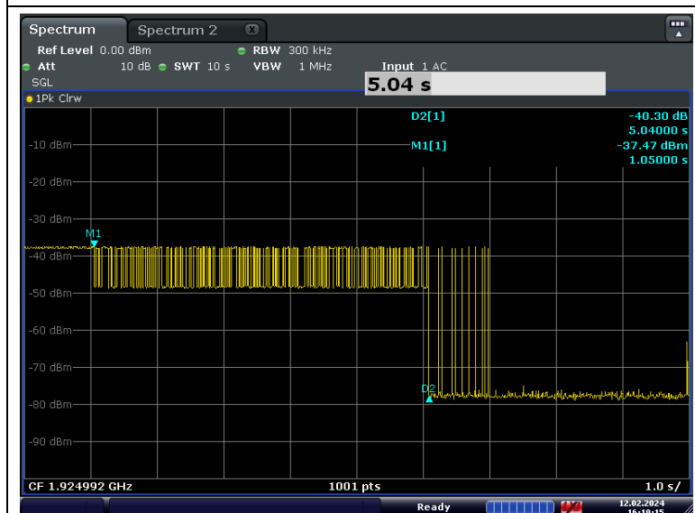
Initial Transmission without Acknowledgements
