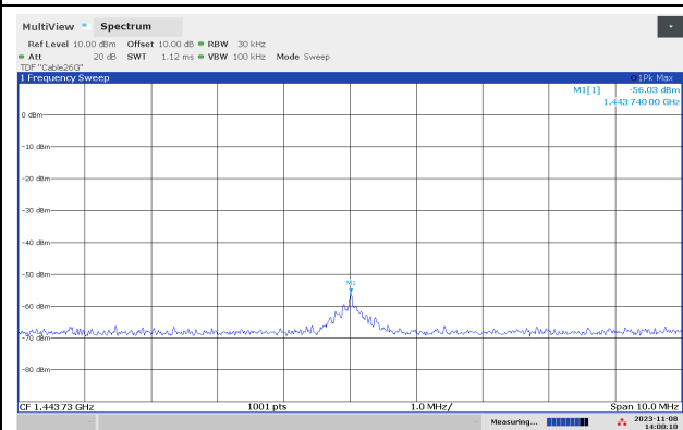
Out-of-Band Emissions 1444 MHz, Middle Channel
