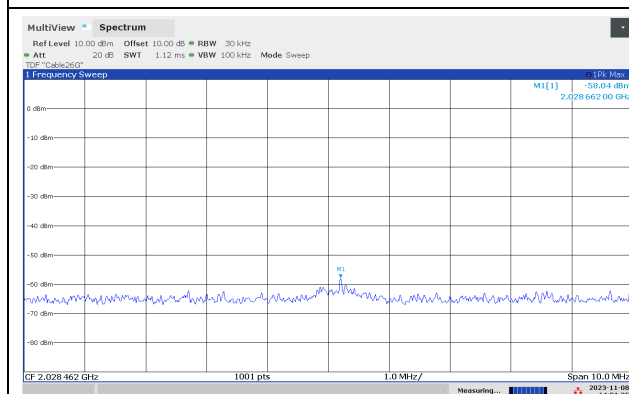
Out-of-Band Emissions 2030 MHz, Middle Channel
