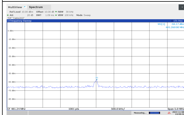
Out-of-Band Emissions 481 MHz, Middle Channel
