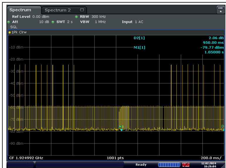
Initial Transmission without Acknowledgements
