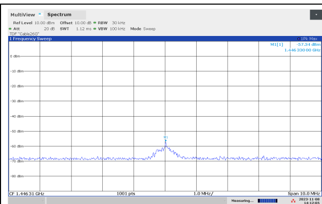
Out-of-Band Emissions 1446 MHz, Upper Channel
