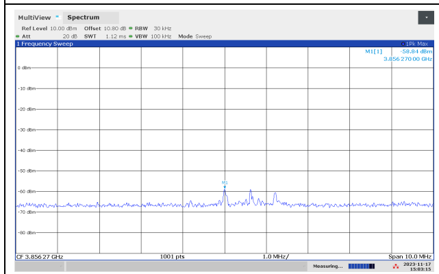
Out-of-Band Emissions 3856 MHz, Lower Channel
