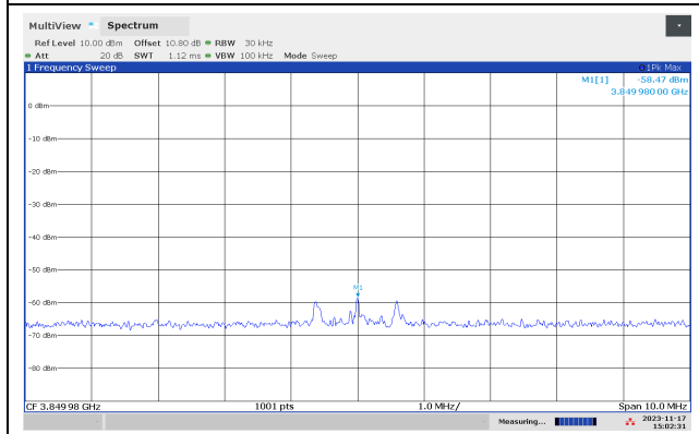
Out-of-Band Emissions 3850 MHz, Lower Channel
