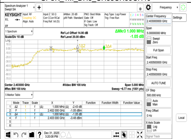
π/4DQPSK_2M_DH5_CH0CH1CH2
