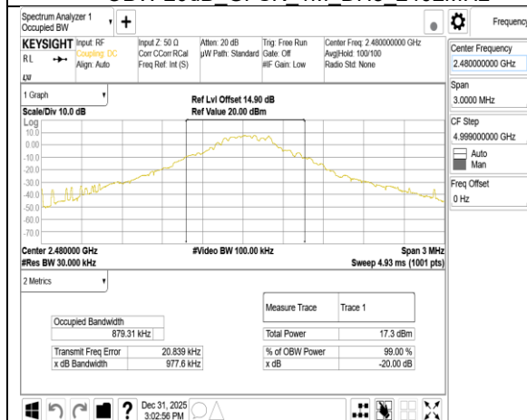
OBW 20dB_GFSK_1M_DH5_2480MHz
