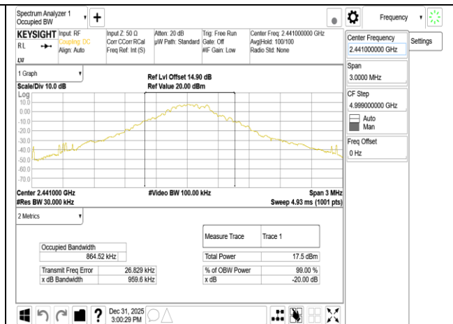
OBW 20dB_GFSK_1M_DH5_2441MHz
