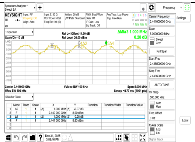
GFSK_1M_DH5_CH38CH39CH40
