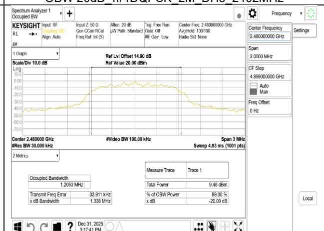
OBW 20dB_pi/4DQPSK_2M_DH5_2480MHz
