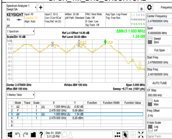
GFSK_1M_DH5_CH76CH77CH78
