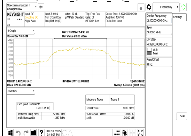
OBW 20dB_pi/4DQPSK_2M_DH5_2402MHz
