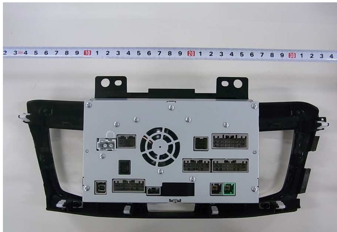
Rear View
