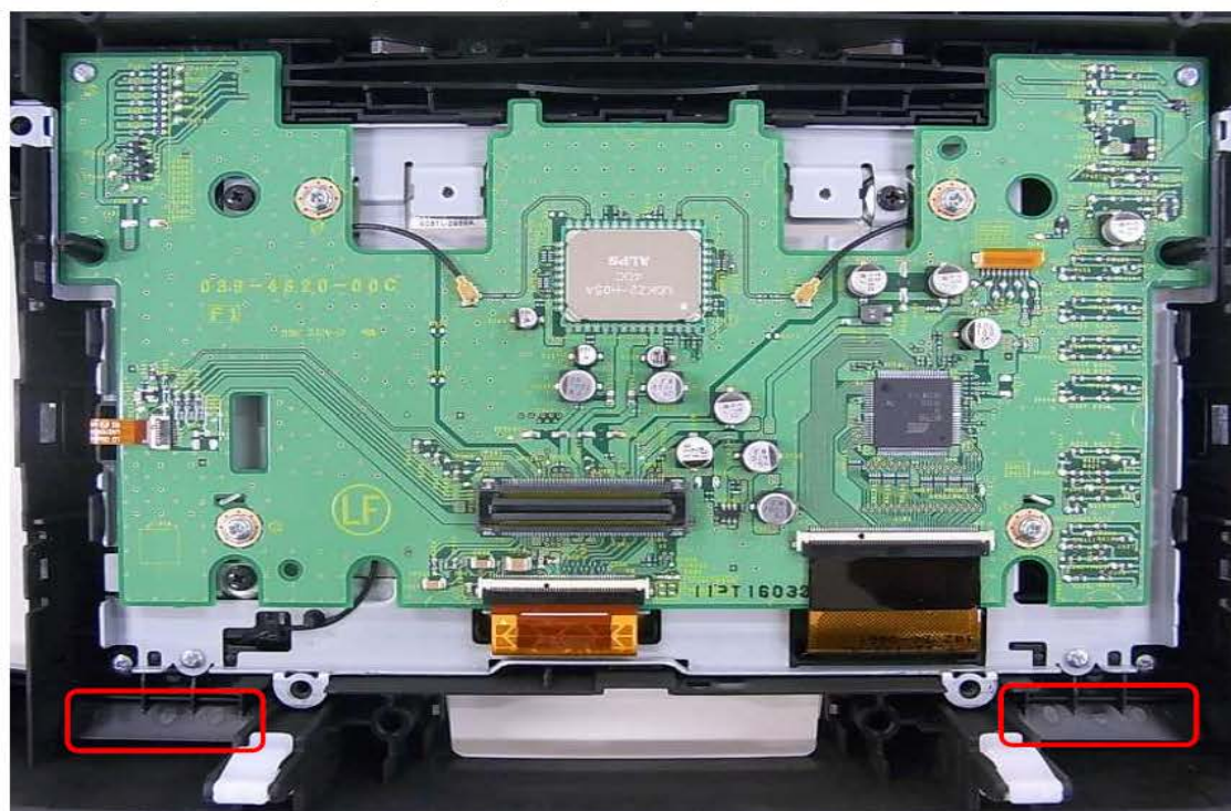
1-2. LCD PCB ASSY - F1 View (more detail)
