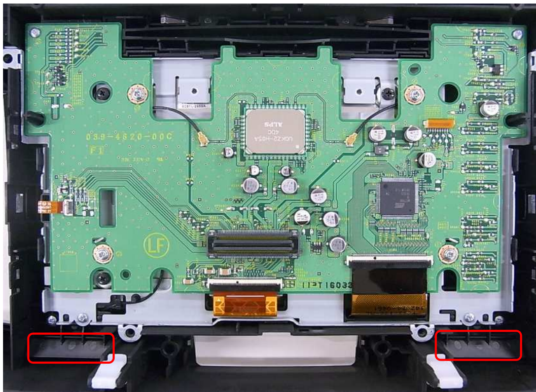
1-2. LCD PCB ASSY - F1 View (more detail)
