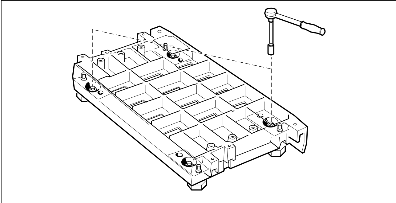
Figure 3-17. Tightening the Base Bolts
