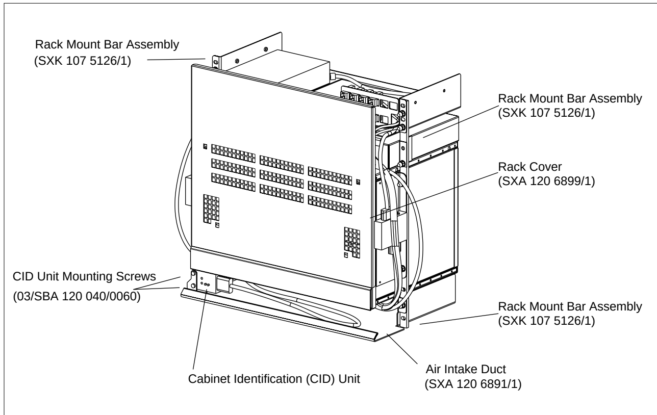
Figure 3-9. CRI Rack Mount
