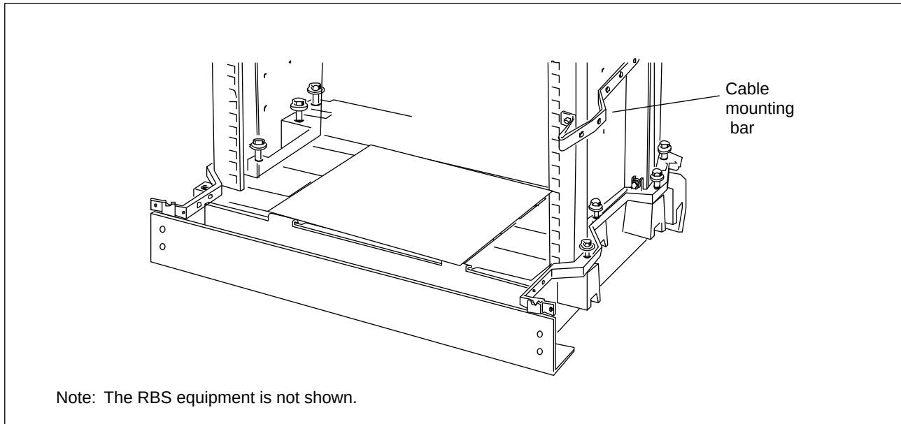
Figure 3-28. Bolting the CRI Cabinet to the Base
