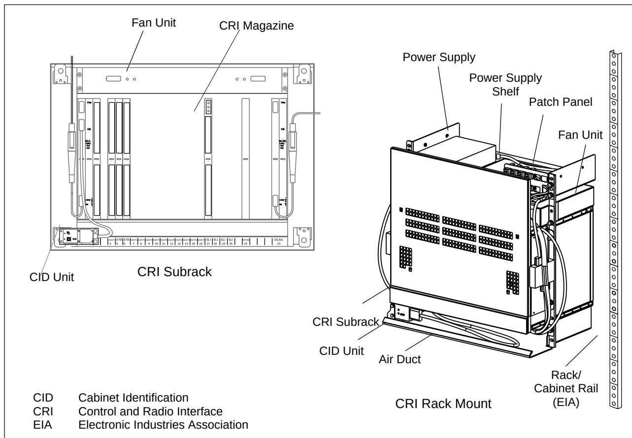
Figure 2-4. CRI Rack Mount Equipment
