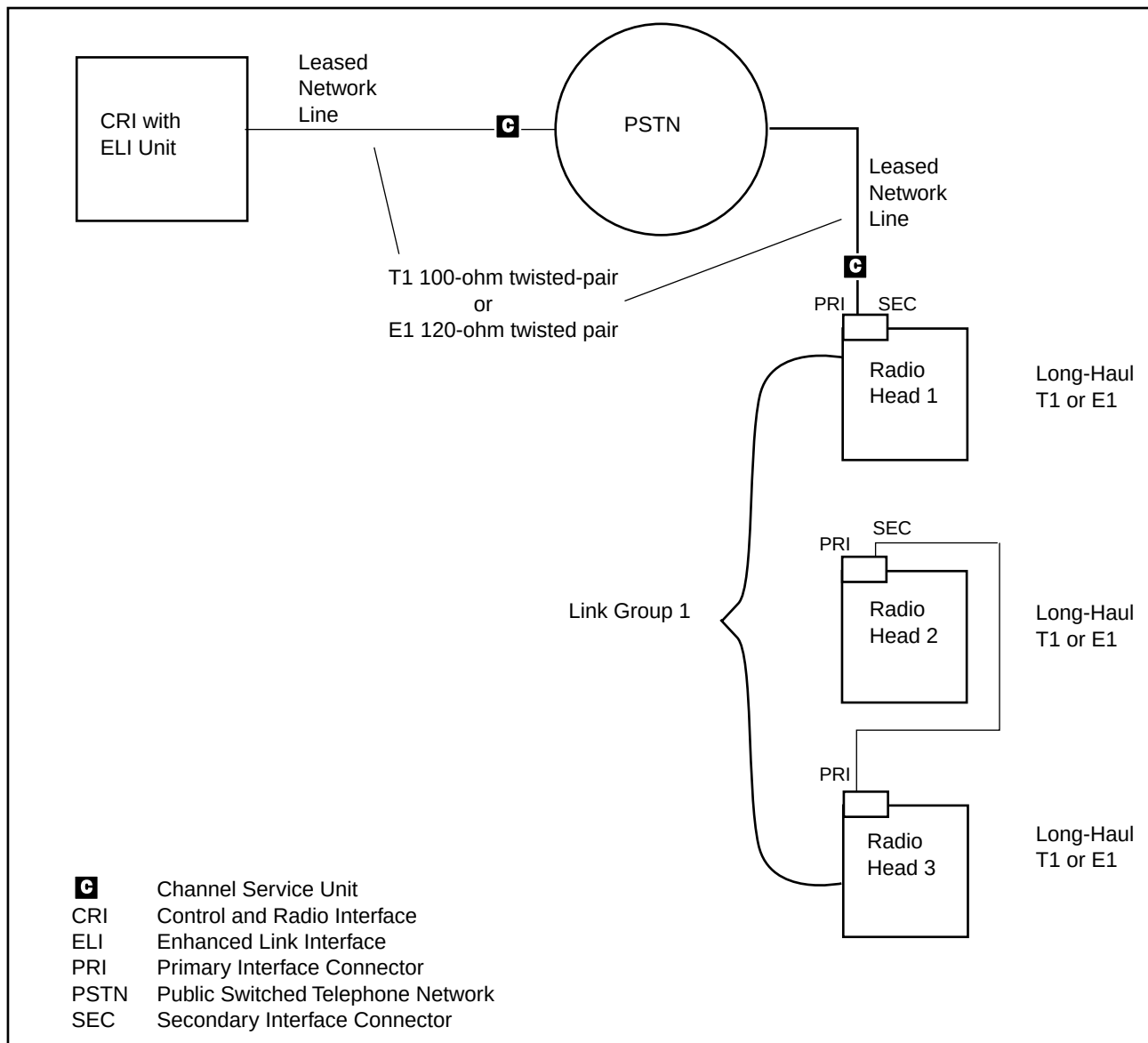
Figure 3-53. T1/E1 PCM Cabling to Radio Heads
