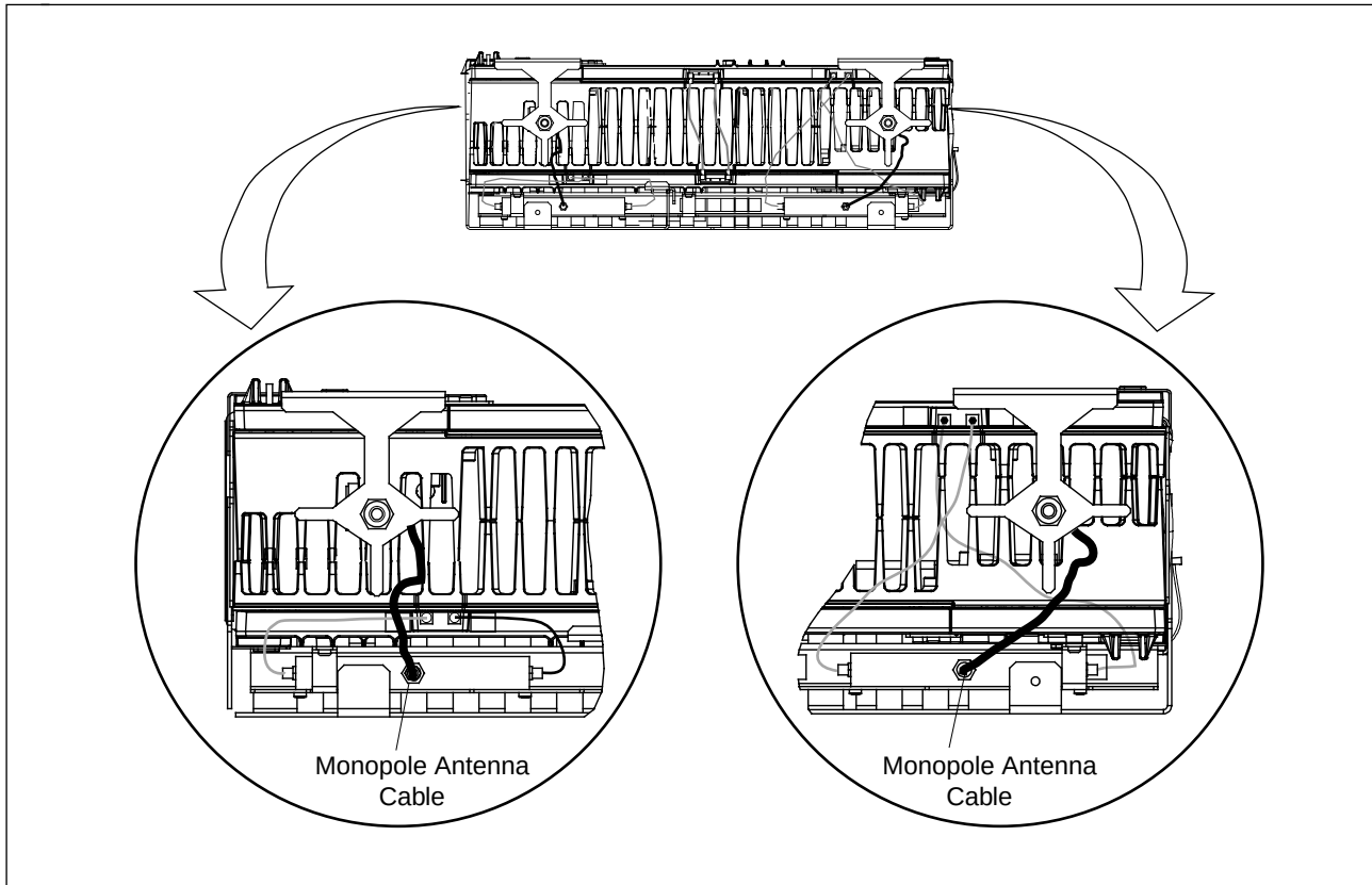
Figure 4-8. Disconnecting the Monopole Antenna Cable
