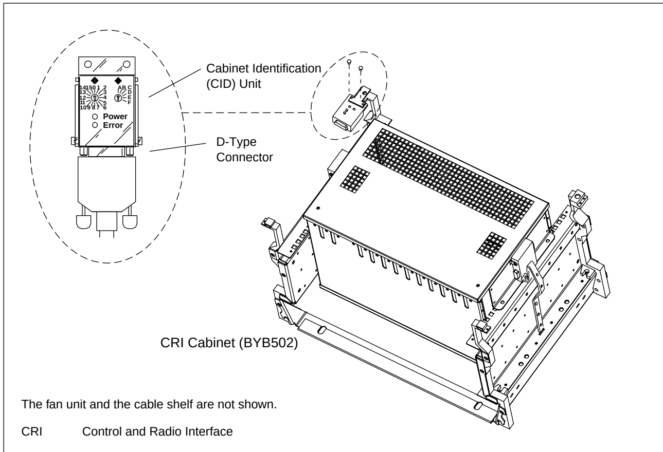
Figure 3-26. CID Unit Installation
