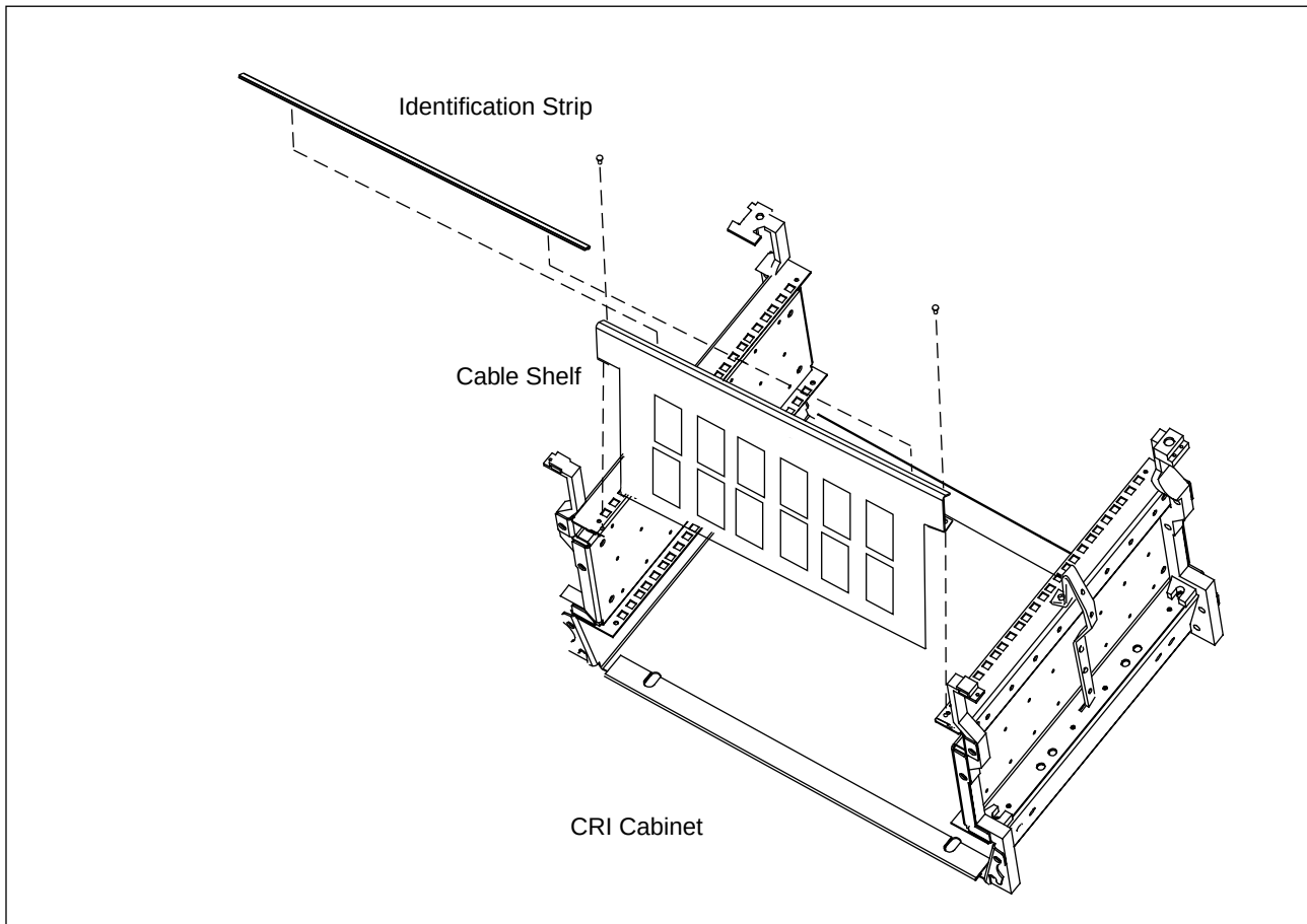
Figure 3-20. Cable Shelf Installation
