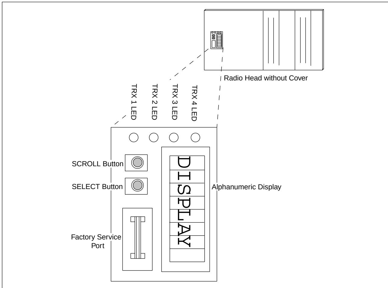
Figure 3-61. Radio Head User Interface
