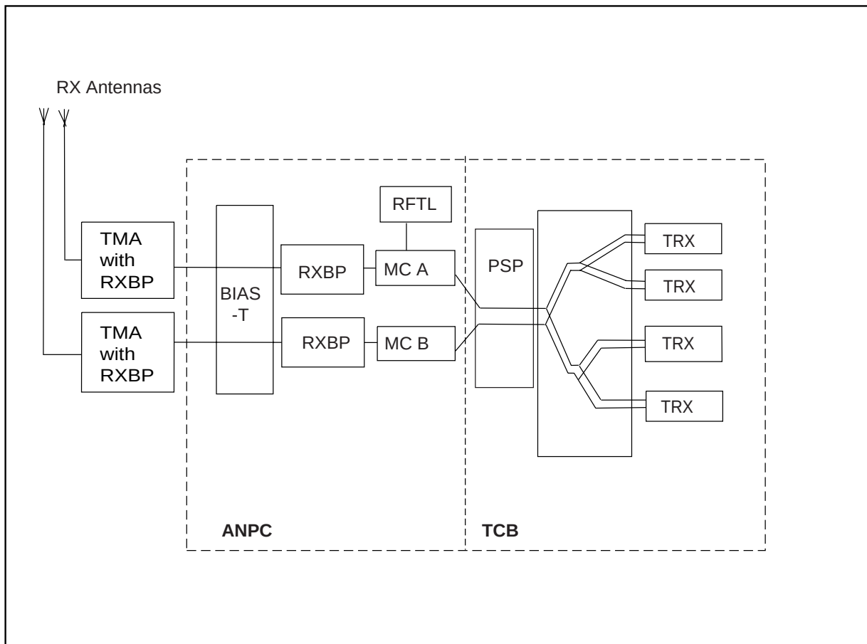
Figure 3-8. Macro with MCPA, 1900 MHz Receive Path
