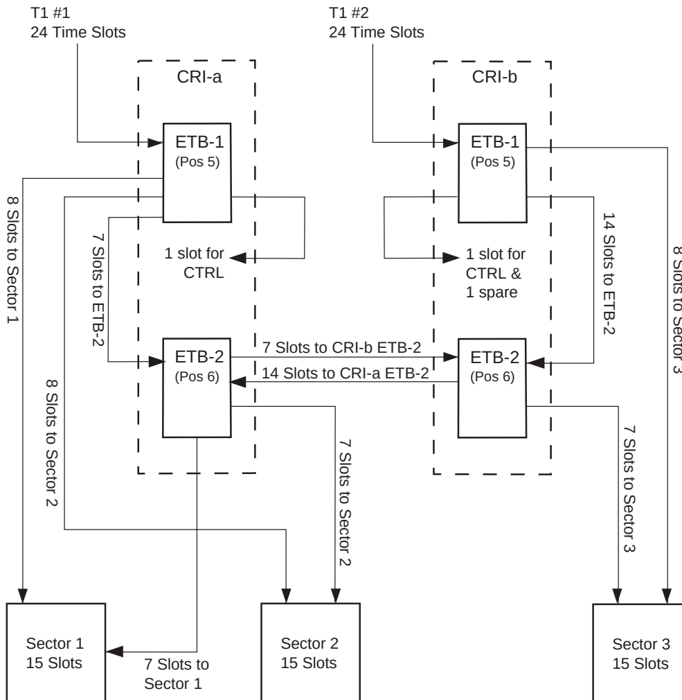
Figure 3-11. 3x15 CRI-PCM (T1) Configuration
