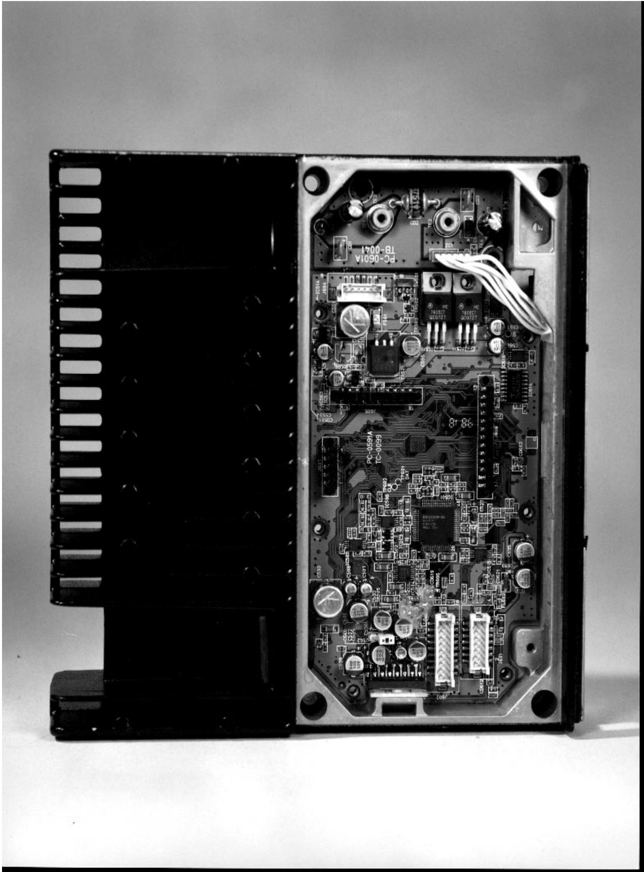
Bottom with Shield removed
