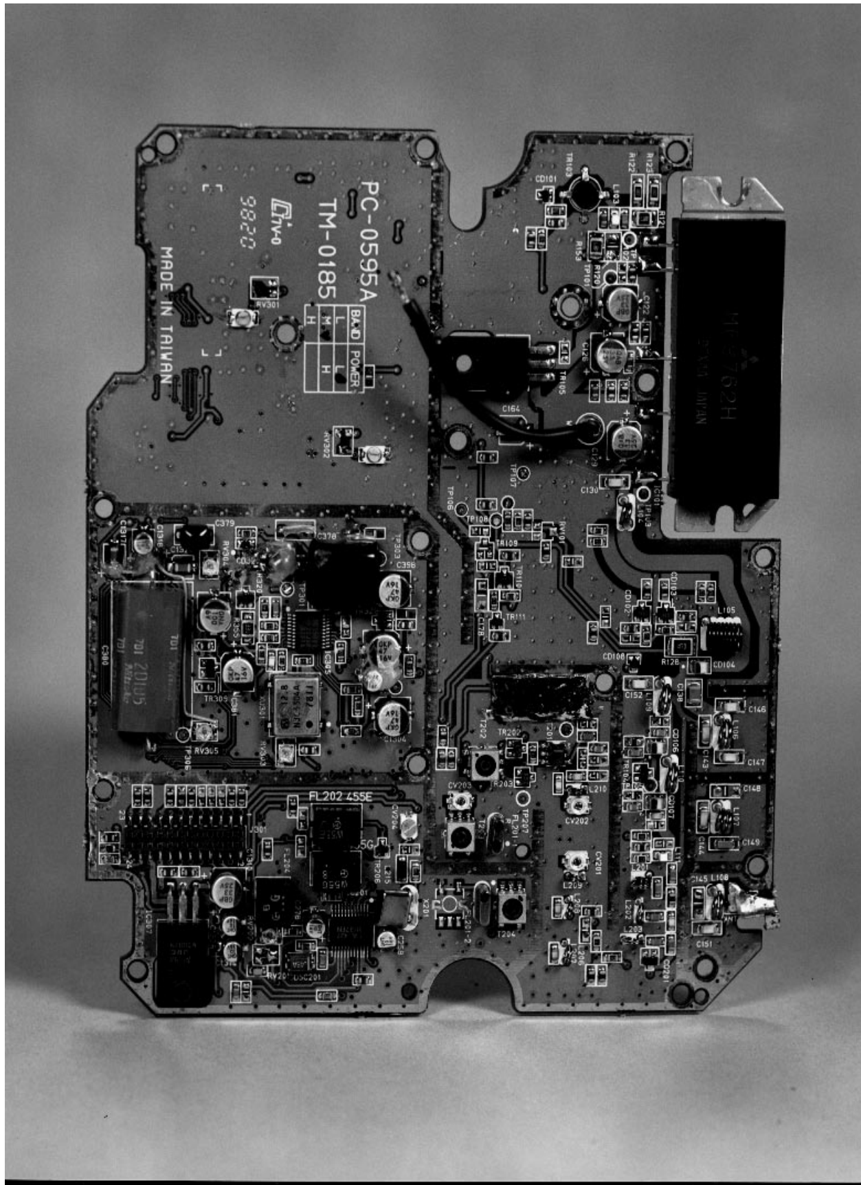
Front of Tx. Board
